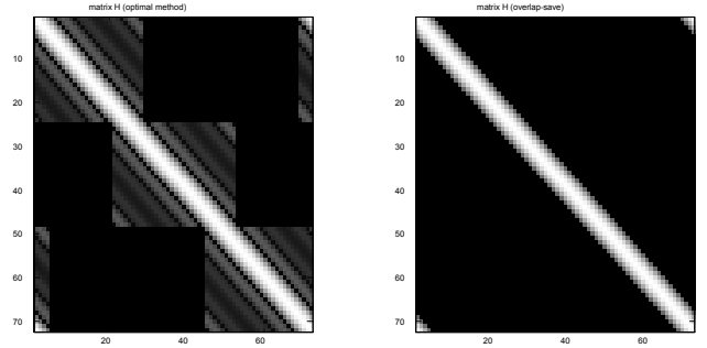
Figure 5: Matrix H (left: optimal method, right: overlap-save).
