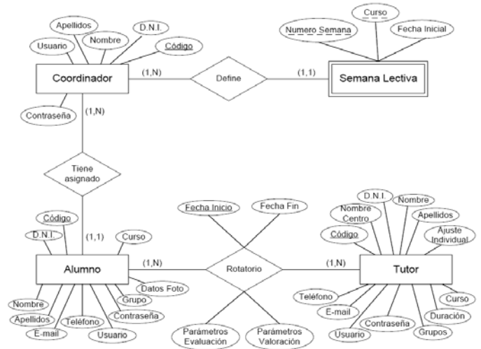
Fig. 3. Relational Model of the database
