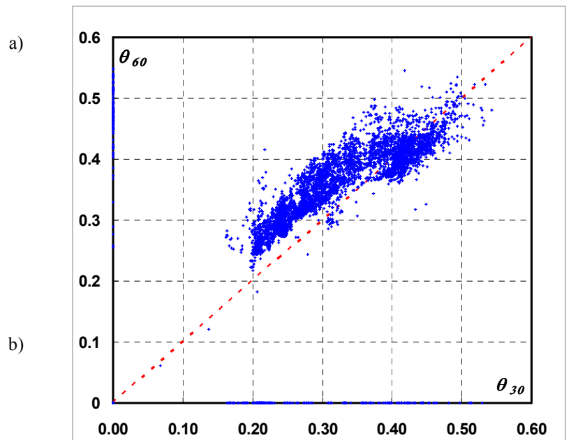
Fig. 6. Values of the mean soil moisture in the deep 60 cm given the soil moisture in the first 30 cm.
