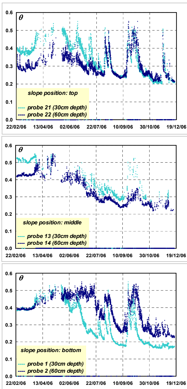
Fig. 5. Temporal variations of the soil moisture at the top, middle and bottom sites.
