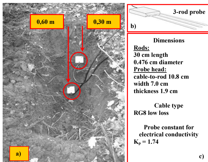
Fig. 3. a) One of the 11 sampling sites with probes at two different depths. b) Schematic representation of a TDR probe. c) General description of the instrumentation.
