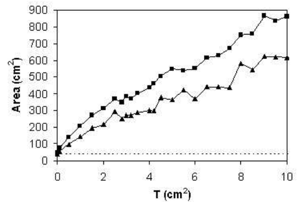
Fig.4 Areas of simulated data for soft boundary ellipse ( a = 4 cm, b = 3 cm) as a function of temperature ( T ). Upper curve was calculated by Fourier analysis of convex surface, lower one is the result of PCA and dashed line shows the area of the basic ellipse.
