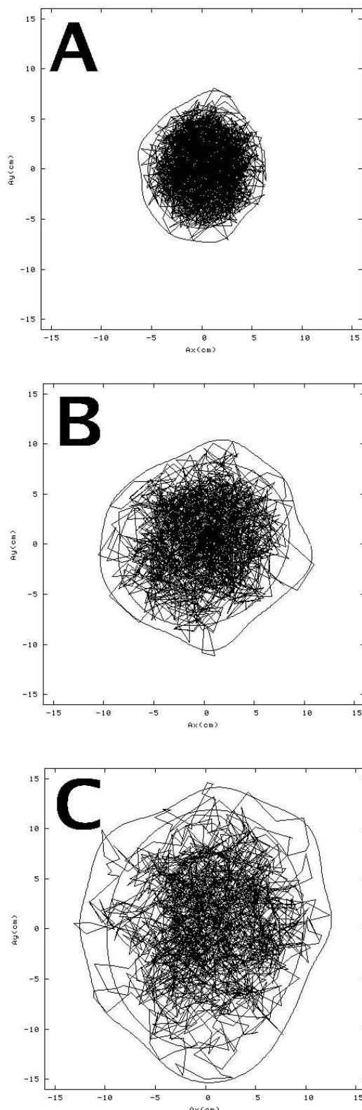
Fig.3 Simulated data for soft boundary ellipse ( a = 4 cm, b = 3 cm, \theta = 80^\circ ) for T = 0.5 (A), 2.0 (B) and 5.0 (C). The outer and inner contours were determined by Fourier and principal component analysis, respectively.
