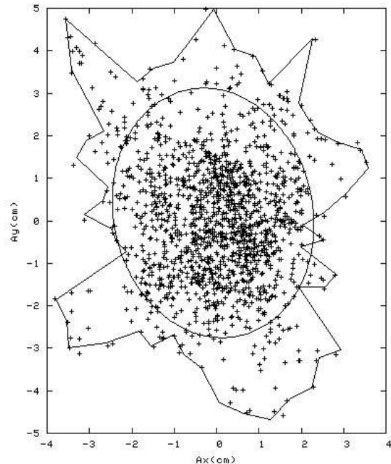
Fig.1 An example of a measured sway area with outline determined by 50 points. The ellipse was determined by PCA.
