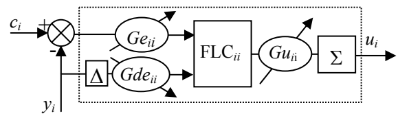
Fig. 5. PI Fuzzy controller.
