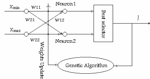
Fig. 3: subnetwork structure.
