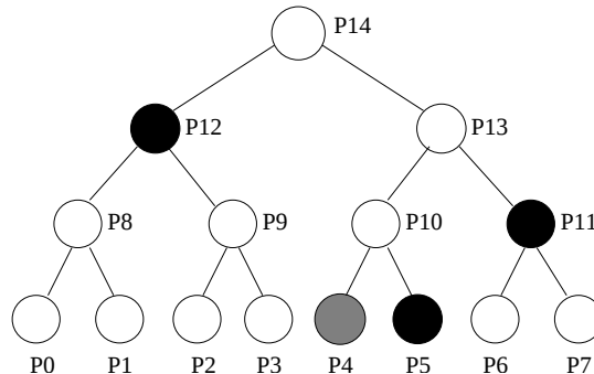
Figure 3: Hash tree
