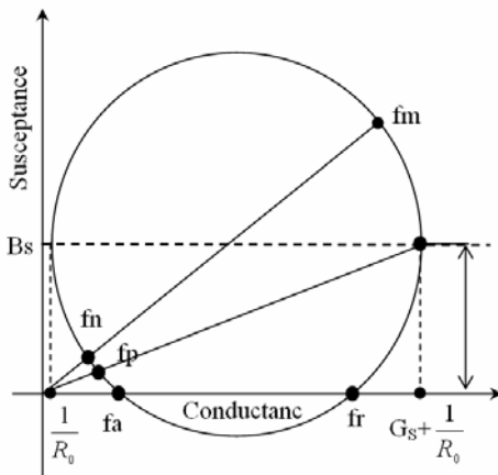
Fig. 5 Complex plane of admittance.
