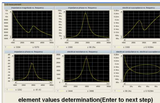
Fig. 10 G-B measurement for unmatching Transducer.
