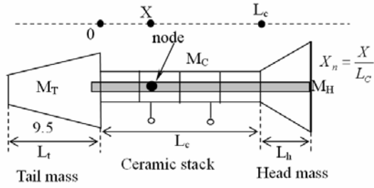
Fig. 1 Tonpiltz transducer cross-section
