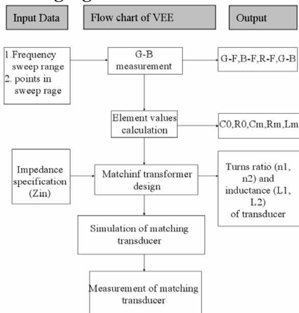
Fig. 8 Flow chart of Agilent VEE Program.
