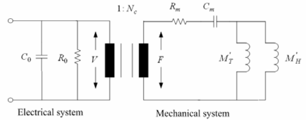
Fig. 3 Equivalent circuit of Tonpiltz transducer working in air.
