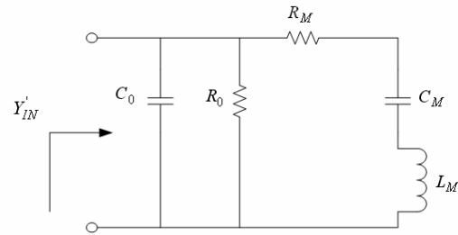
Fig. 4 Simplified equivalent circuit of Tonpiltz transducer.
