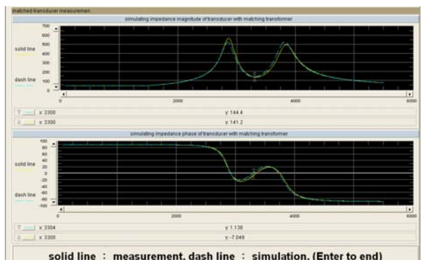
Fig. 11 Matching transducer measurement.
