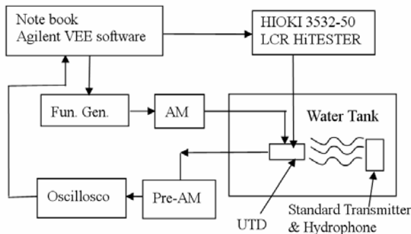
Fig. 7 Diagram of PC_base Measurement System.
