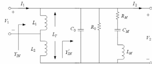
Fig. 6 Equivalent circuit of Tonpiltz transducer with matching transformer.
