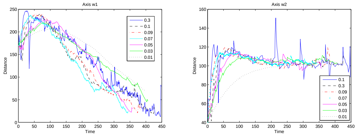
(c) Step (synapses) convergence for w_1 with diverse step sizes. (d) Step (synapses) convergence for w_2 with diverse step sizes.
