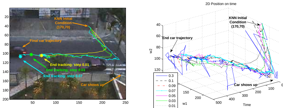
(a) Resulting tracking for diverse step sizes.
