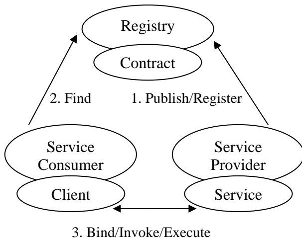
Figure 1: Publish-Find-Bind-Execute paradigm
