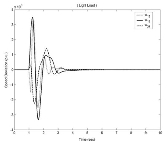
Fig. 11 Dynamic response for \Delta\omega_{12} , \Delta\omega_{34} , \Delta\omega_{13} considering transitory 3-phase fault at bus-7 of three cycles duration for light loading conditions with GFLPSS.
