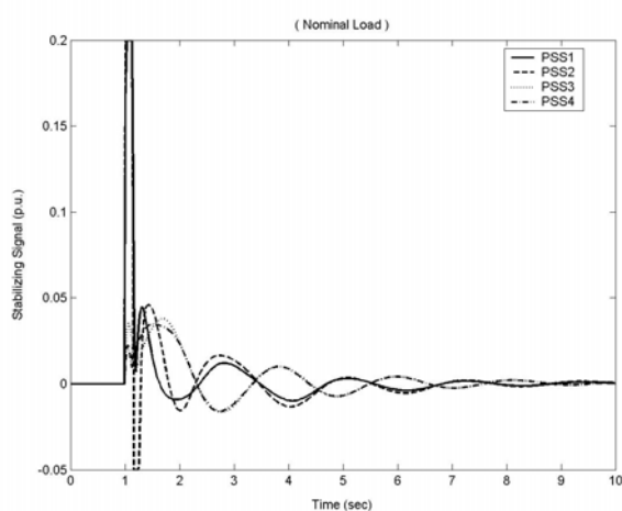
Fig. 14 Stabilizing signal under three-phase fault with CPSS.
