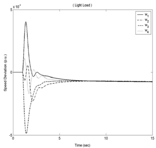
Fig. 7 Dynamic response for \Delta\omega_1 , \Delta\omega_2 , \Delta\omega_3 and \Delta\omega_4 considering V_{ref} 1 = -0.05 p.u. and V_{ref} 3 = 0.05 p.u. for light loading conditions with GFLPSS.
