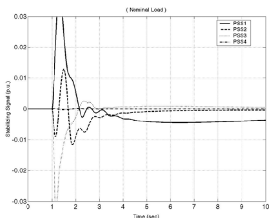
Fig.13 Stabilizing signal under small perturbation with GFLPSS.
