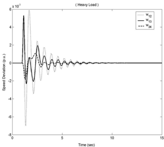
Fig.9 Dynamic response considering transitory 3-phase fault at bus-7 of three cycles duration for heavy loading conditions with GFLPSS.
