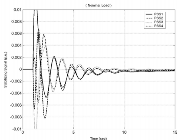
Fig. 12 Stabilizing signal under small perturbation with CPSS.
