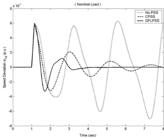
Fig. 8. Dynamic response for \Delta\omega_{13} following three phase, 3-cycle fault at bus-7 of for nominal loading conditions (Interarea mode).
