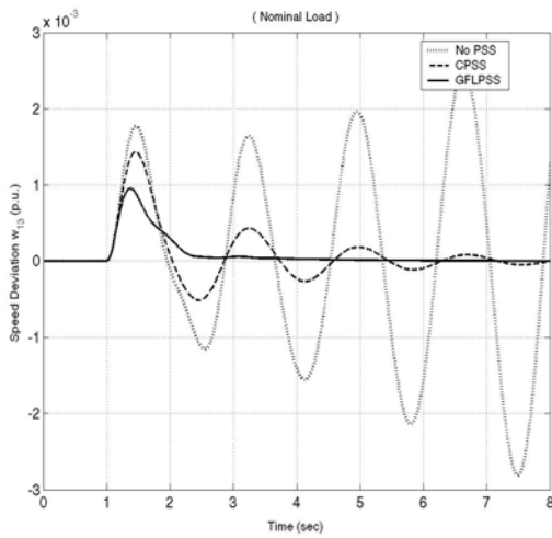
Fig. 4 Dynamic response for \Delta\omega_{13} considering \Delta V_{ref} 1 = -0.05 p.u. and \Delta V_{ref} 3 = 0.05 p.u. for nominal load (local mode).
