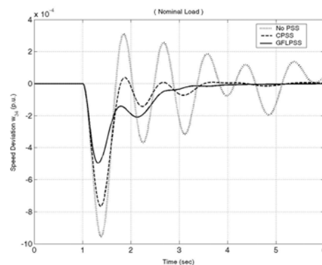
Fig. 3 Dynamic response for \Delta \omega_{34} considering \Delta V_{ref 1} = - 0.05 p.u. and \Delta V_{ref 3} = 0.05 p.u. for nominal load (local mode).
