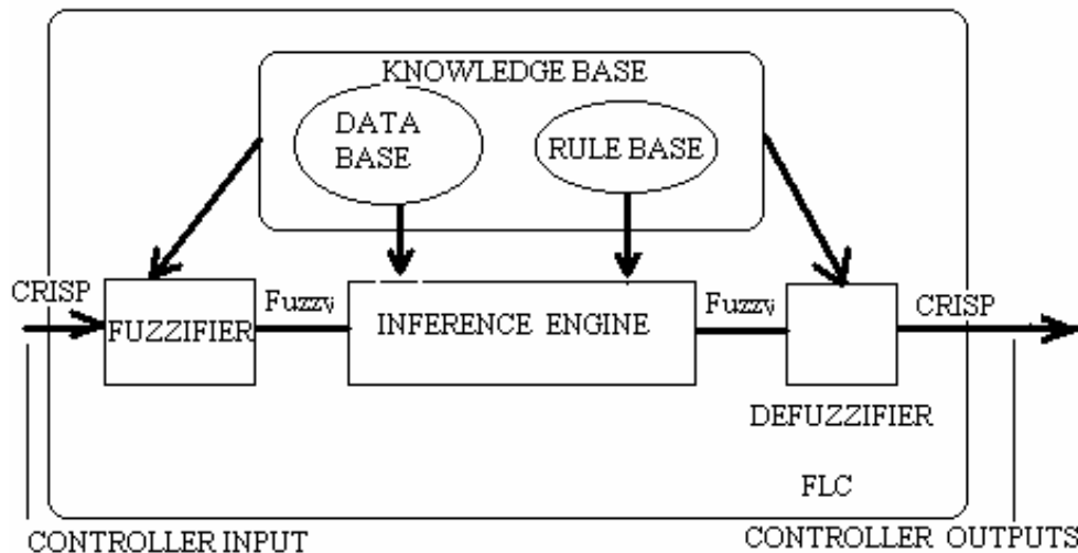
Fig.1. Block Diagram of Fuzzy Logic Controller
