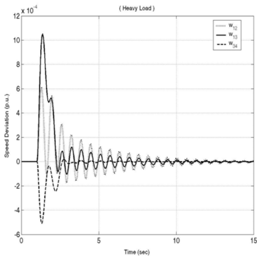
Fig. 5 Dynamic response for \Delta\omega_{12} , \Delta\omega_{34} , \Delta\omega_{13} considering \Delta V_{ref} 1 = -0.05 p.u. and \Delta V_{ref} 3 = 0.05 p.u. for heavy load conditions with GFLPSS.
