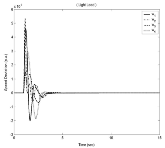
Fig. 10 Dynamic response for \Delta\omega_1 , \Delta\omega_2 , \Delta\omega_3 and \Delta\omega_4 considering transitory 3-phase fault at light loading conditions with GFLPSS.
