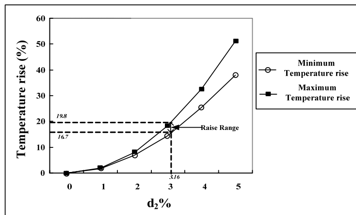
Fig. 5 Winding temperature rise due to voltage imbalance
