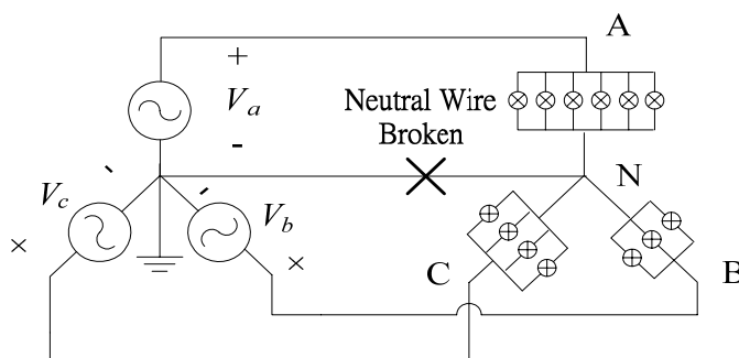
Fig. 2 Schematic diagram of a 3 \phi 4W system with broken neutral wire
