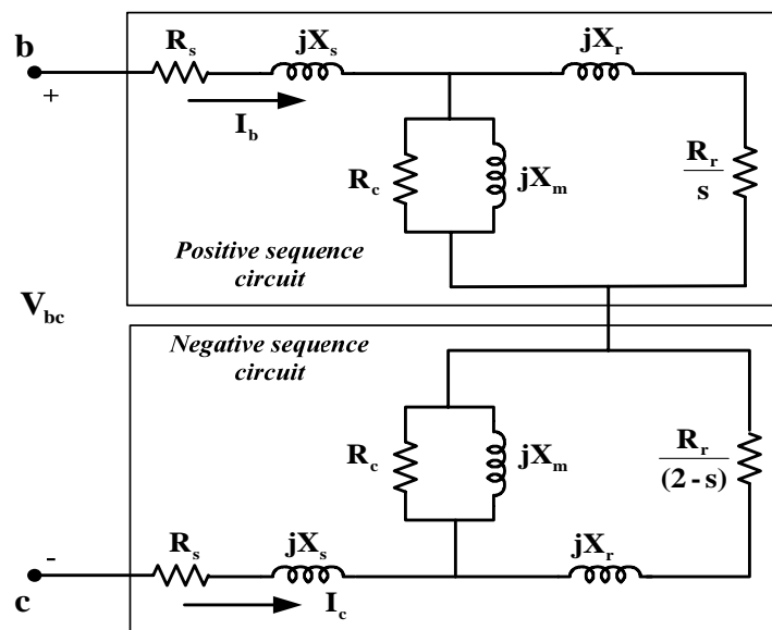
Fig. 9 Equivalent sequence circuit of single-phase operation of a three-phase induction machine
