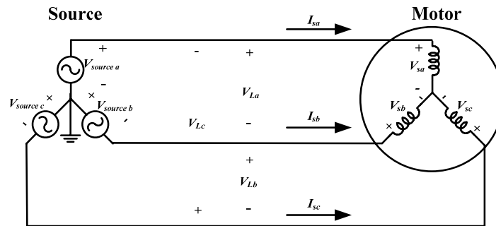
Fig. 7 Three phase motor fed by a balanced power supply system
