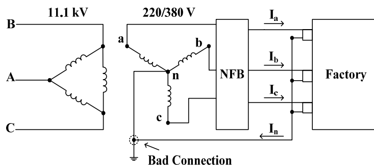
Fig. 1 Power supply system for a three-floor building housing a small factory
