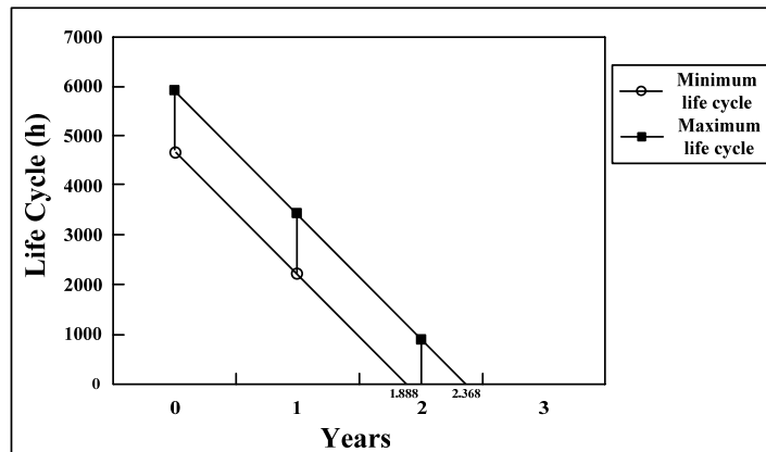
Fig. 6 Motor life cycle reduction under VUR of 3.163%
