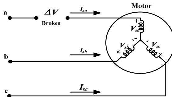
Fig. 8 Single-phase operation of a three-phase motor
