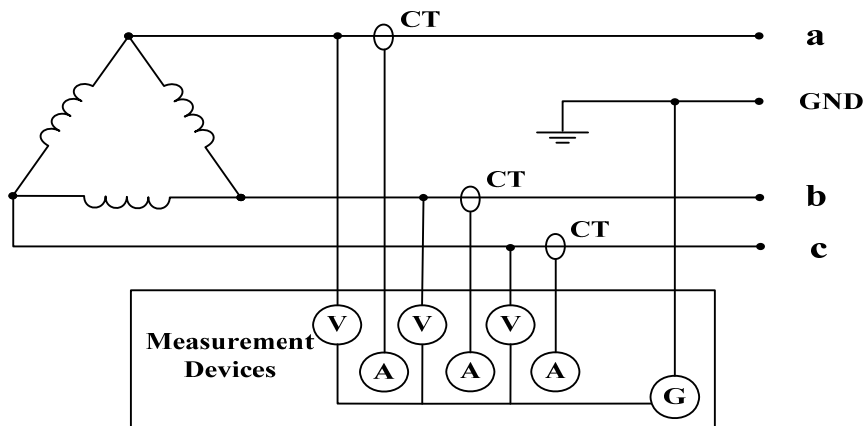
Fig. 4 Schematic diagram for measure voltage imbalance of a three phase motor
