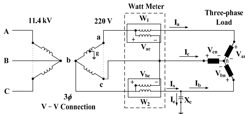
Fig. 3 Schematic diagram for the case study of unsuitable capacitor bank installation
