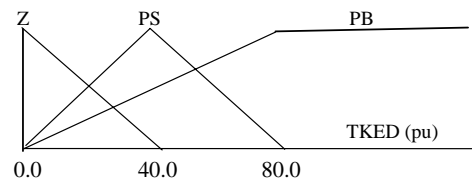
Fig. 5. Membership functions of TKED.
