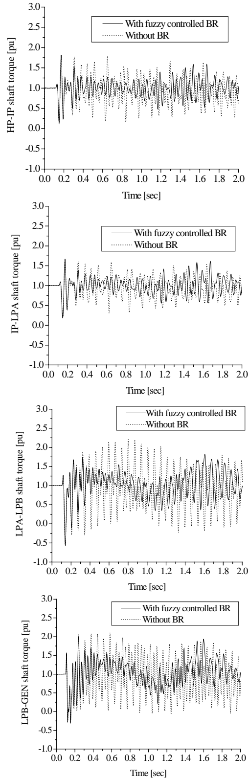
Fig. 7. Shaft torsional torque responses of generator G1 for 3LG fault at point A considering a communication delay of 20 msec.
