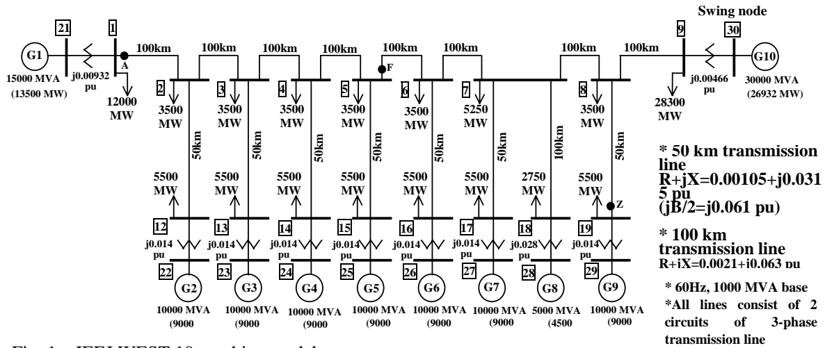
Fig. 1. IEEJ WEST 10-machine model system.
