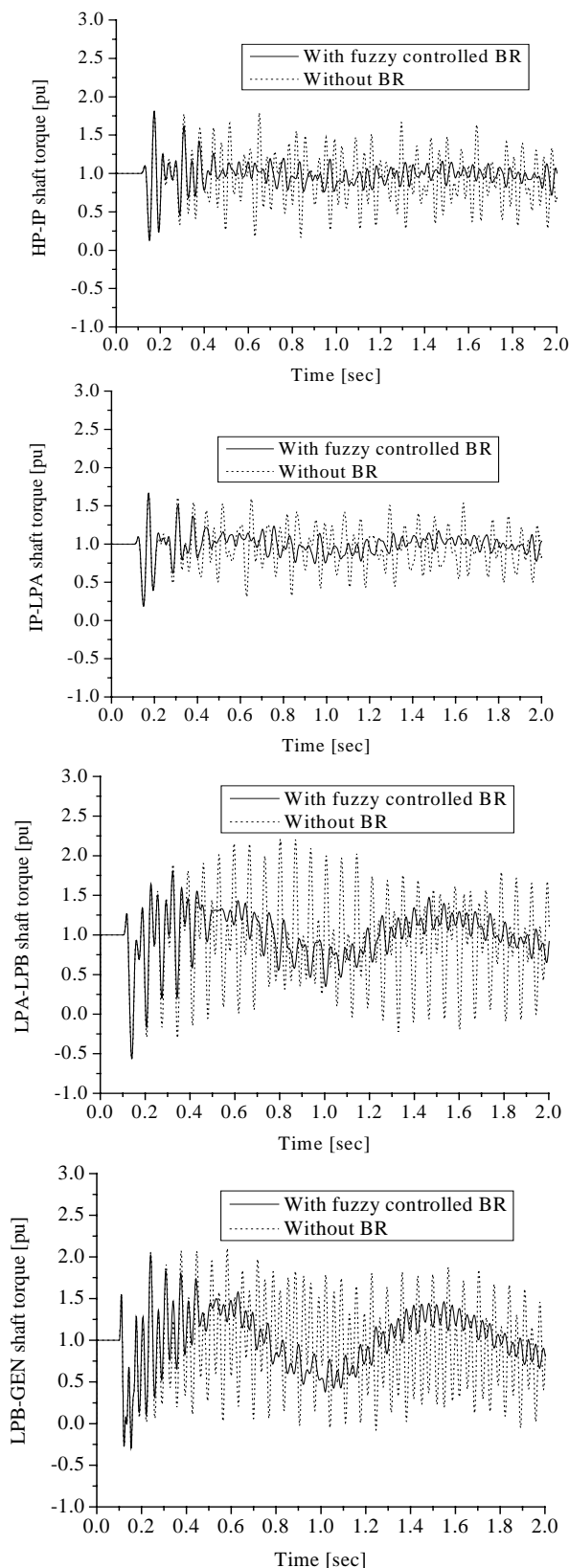
Fig. 8. Shaft torsional torque responses of generator G1 for 3LG fault at point A using prediction function method and considering a communication delay of 20 msec.
