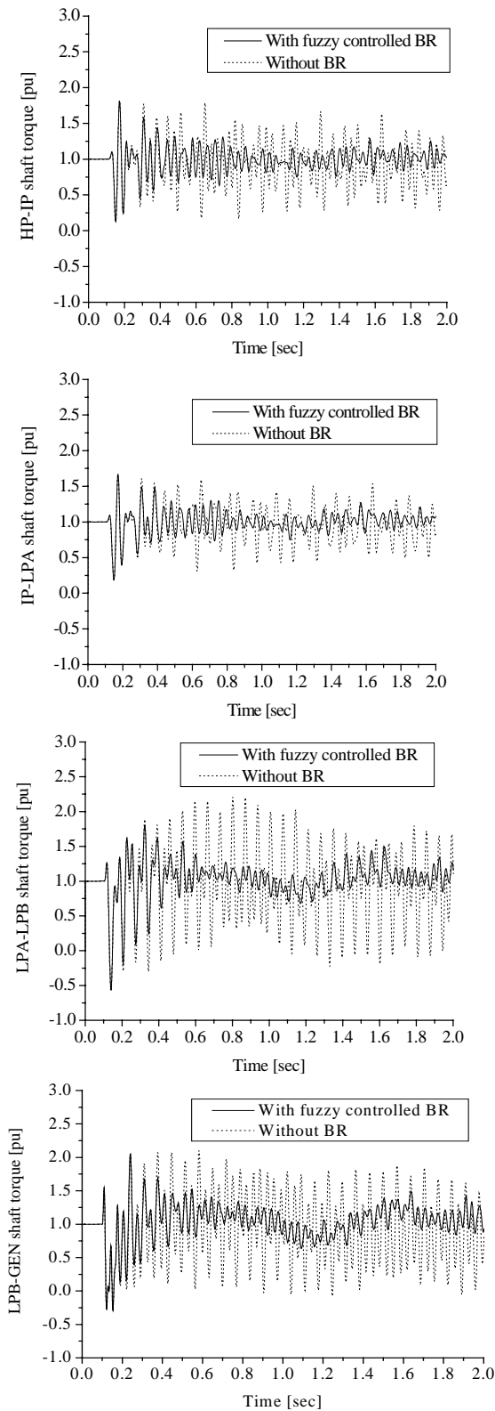
Fig. 6. Shaft torsional torque responses of generator G1 for 3LG fault at point A without considering communication delay.
