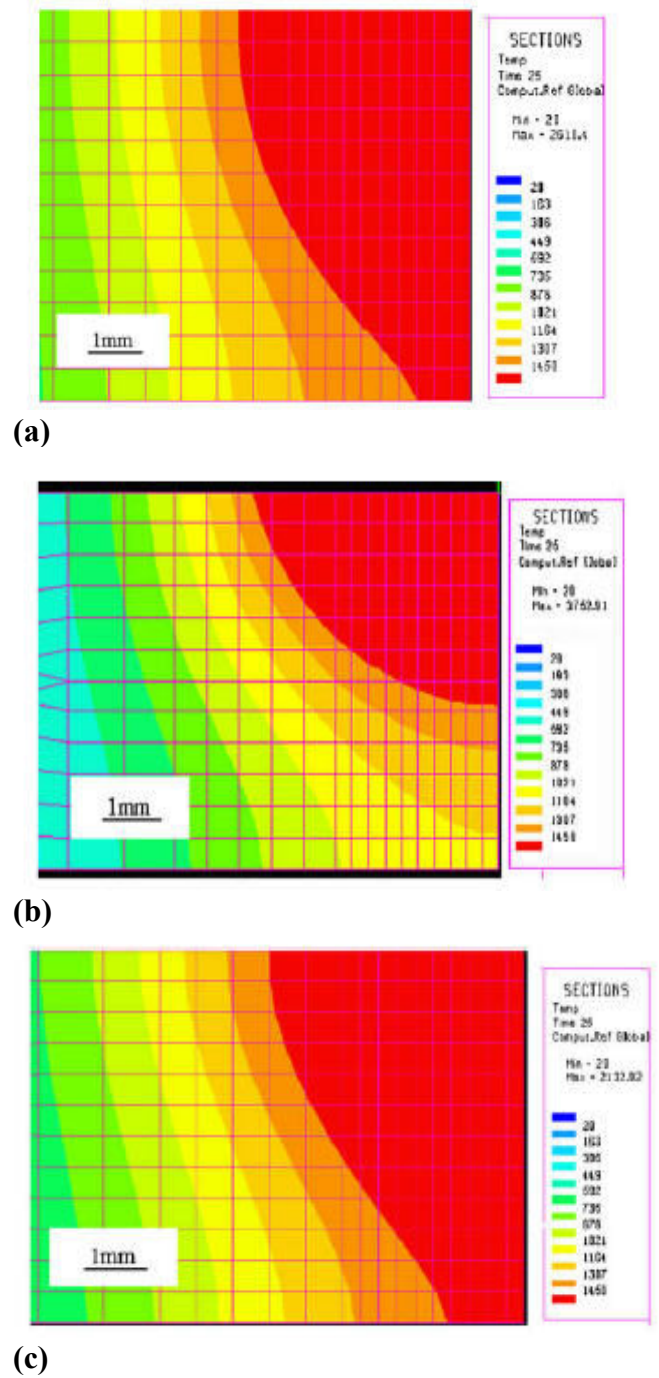
Fig.8. Two-dimensional distributions of temperature and flow velocity in (a)argon, (b)helium (c)carbon dioxide gas.
