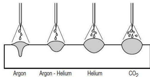
Fig.9. Bead contour and penetration patterns for various gases
