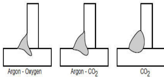
Fig.10. Relative effect of Oxygen versus CO 2 additions to the argon gas
