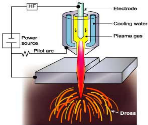
Fig.1. Plasma Arc Cutting Process
