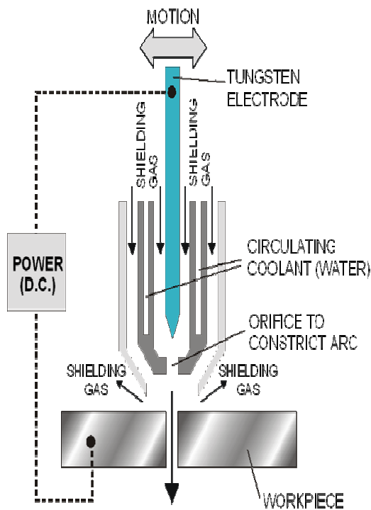
Fig.2. Plasma jet
