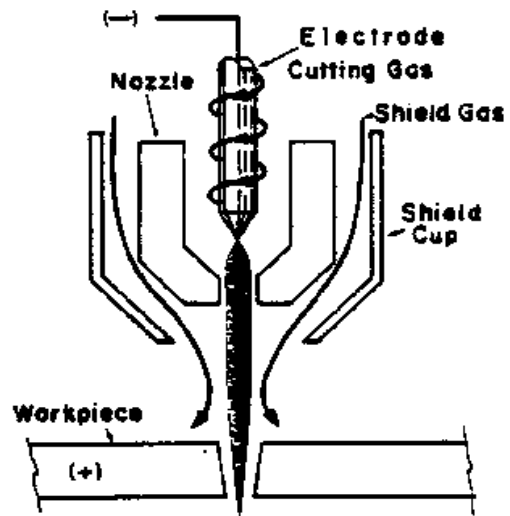
Fig.5. Dual Flow Plasma Cutting
