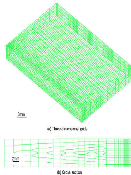
Fig3. Finite-Element modeling
