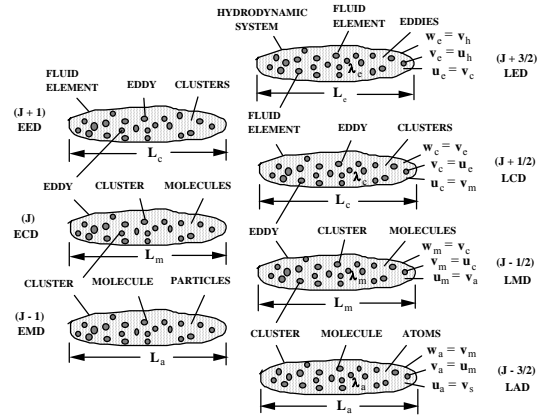
Fig.2 Hierarchy of statistical fields for equilibrium eddy-, cluster-, and molecular-dynamic scales and the associated laminar flow fields.
