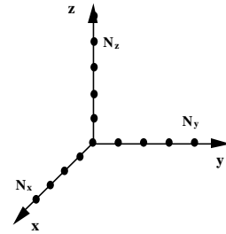
Fig.3 Discrete Cartesian coordinates in three-dimensional Euclidean space.
