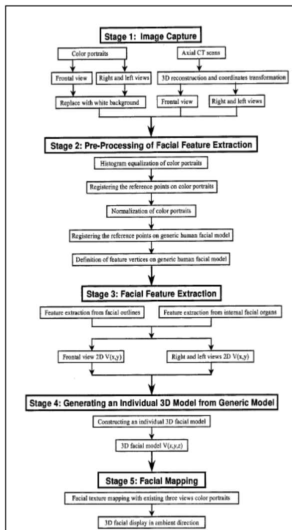
Fig 5. Steps in Facial Model Generation [28]
