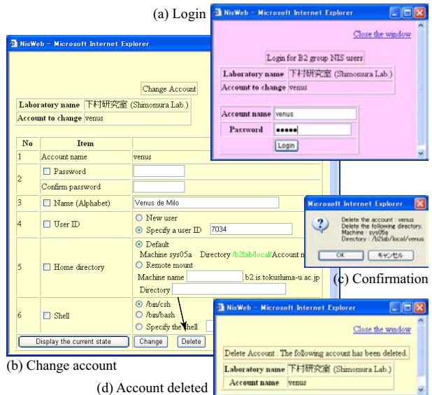
Figure 7: Account deletion page
