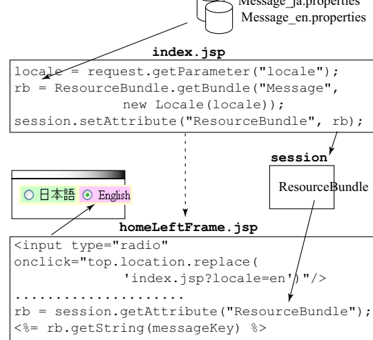
Figure 10: Session-based switching method of languages
