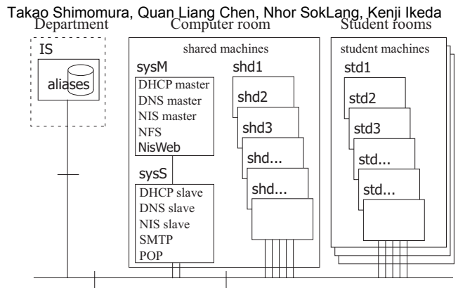
Figure 1: Laboratory network configuration
