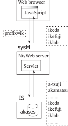
Figure 8: Unique account name input method
