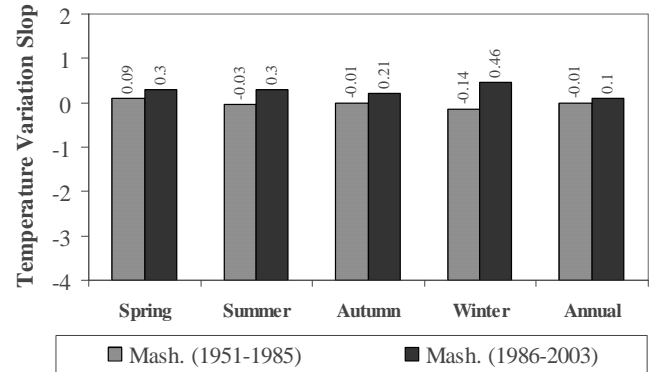
Figure 5 – The comparison of seasonal and annual temperature variation slopes in town of Mashhad for years of 1951-1985 and 1986-2003.
