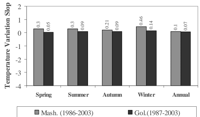
Figure 6 – The comparison of seasonal and annual temperature variation slopes for Mashhad and Golmakan stations in 1986 to 2003.
