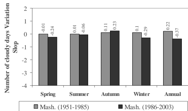
Figure 12 – The comparison of seasonal and annual number of cloudy days’ variation slopes in town of Mashhad for years of 1951-1985 and 1986-2003.
