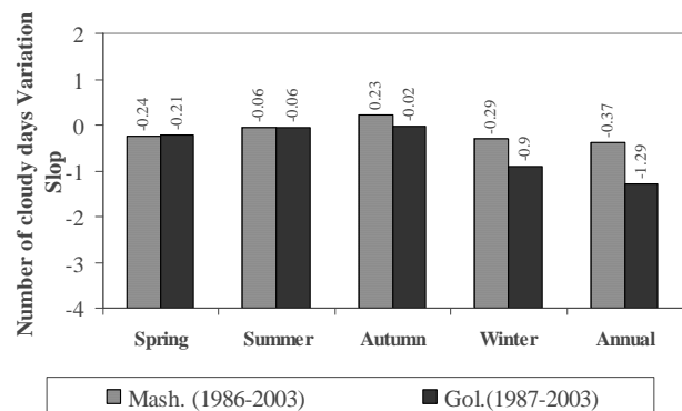
Figure 13 – The comparison of seasonal and annual number of cloudy days’ variation slopes in Mashhad and Golmakan stations (1986-2003).
