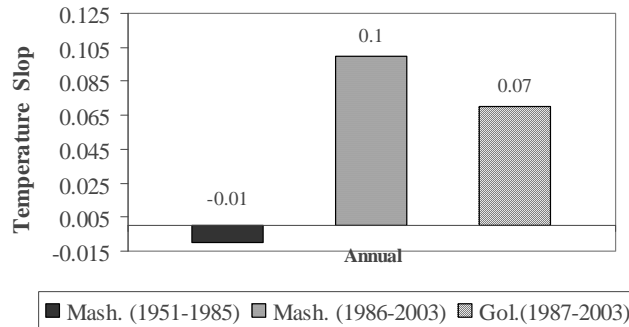
Figure 14 – The comparison of annual temperature variation slopes in Mashhad for years of 1951-1985 and 1986-2003, and Golmakan stations for 1986-2003.
