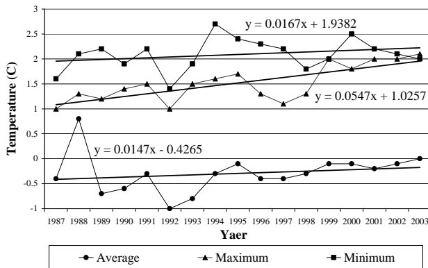
Figure 4 - UHI Index for Mashhad Station
