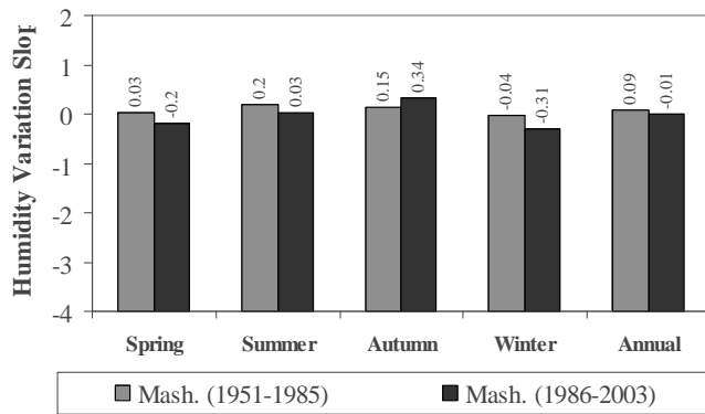
Figure 10 – The comparison of seasonal and annual humidity variation slopes in city of Mashhad for years of 1951-1985 and 1986-2003.
