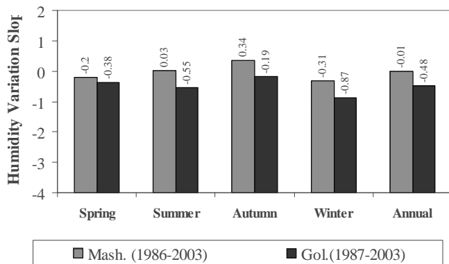
Figure 11 – The comparison of seasonal and annual humidity variation slopes in Mashhad and Golmakan stations (1986-2003).
