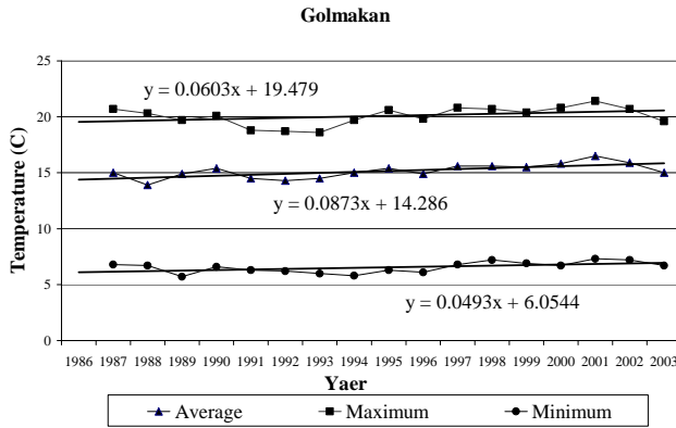
Figure 3 - Temperature Variation at Golmakan Station
