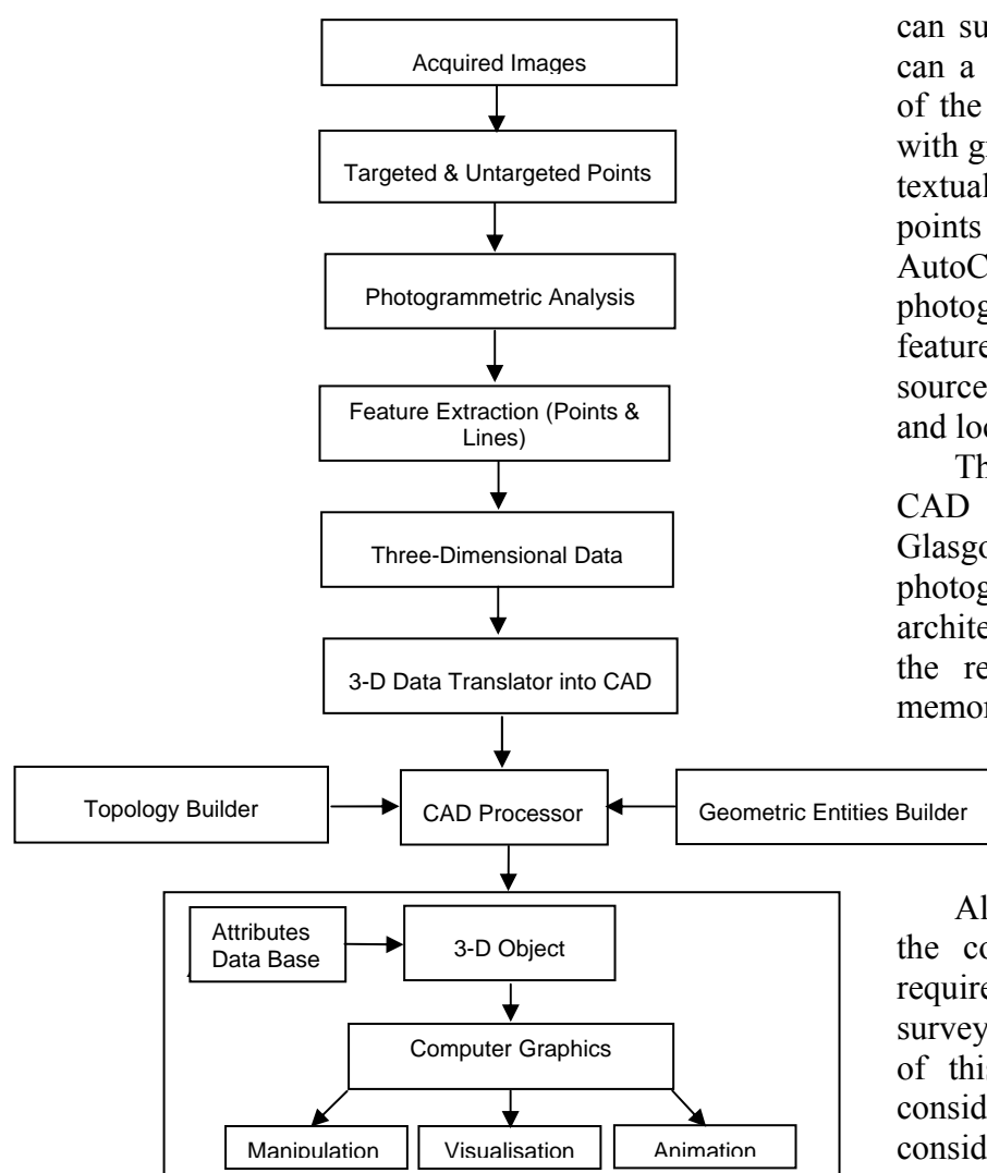
Fig. 1. An Overview of Archaeological and Architectural Information System
