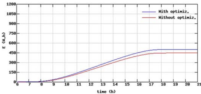
Fig. 6 Daily energy generation
