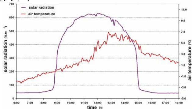
Fig. 2 Behaviour of solar radiation intensity in December 2005
