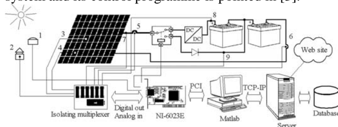
Fig. 4 Connection and positron of measuring sensor
