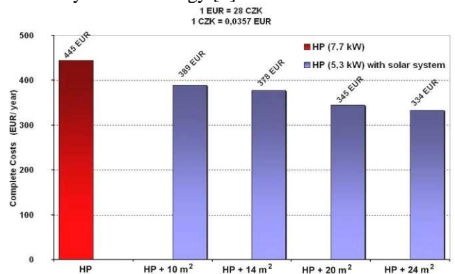
Fig. 10 Confrontation of operating costs
