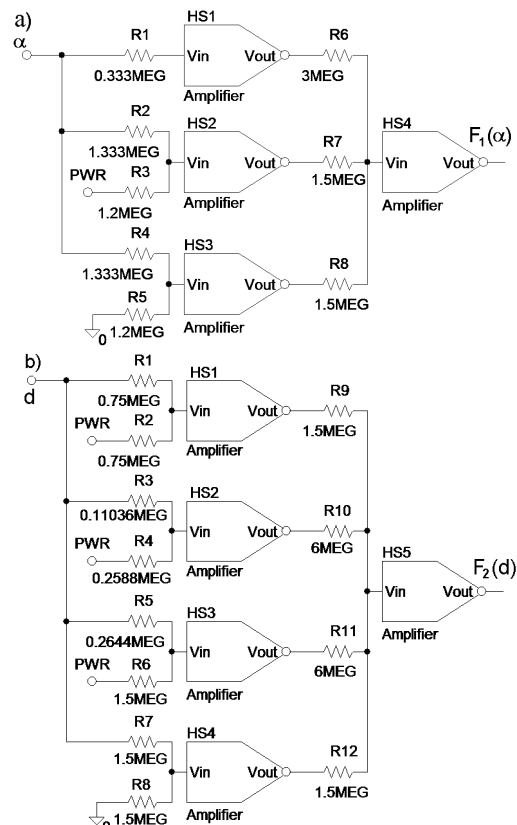
Fig.45 Fuzzifier schematics a) for the angle and b) for the distance.
