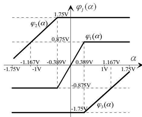
Fig.41 Component functions for the function represented in Fig.40.
