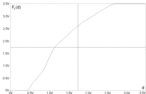
Fig.47 Output of the fuzzifier shown in Fig.45(b) and derived by SPICE simulation.
