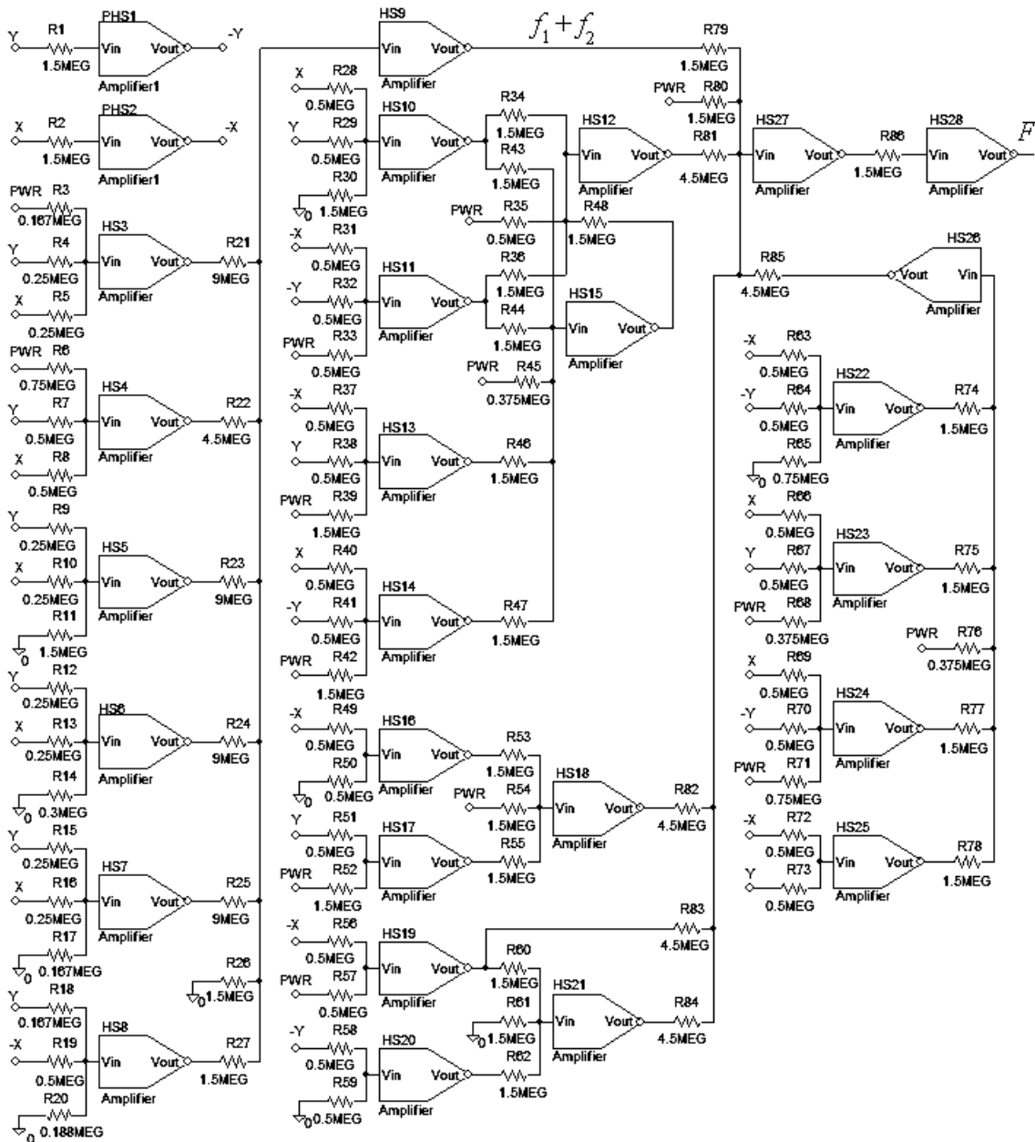
Fig.36 The controller schematic for experiments.
