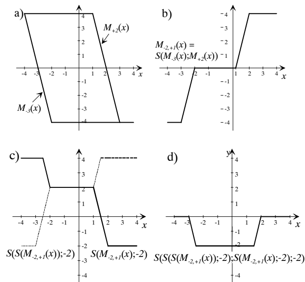
Fig.15 Example of mask-functions application.
