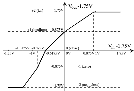
Fig.42 Piecewise-linear fuzzification function for the variable distance .
