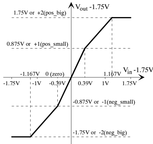
Fig.40 Piecewise-linear function for fuzzification of the variable angle .
