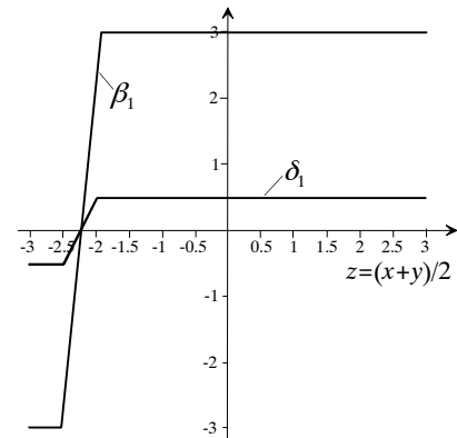
Fig.23 Representation of the function \alpha_1(z) .
