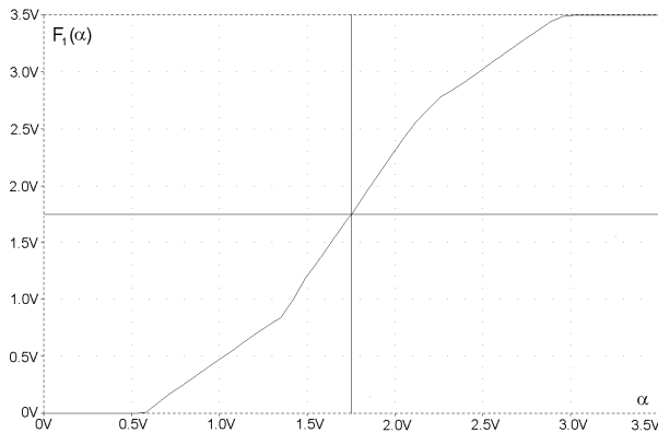
Fig.46 Output of the fuzzifier shown in Fig.45(a) and derived by SPICE simulation.
