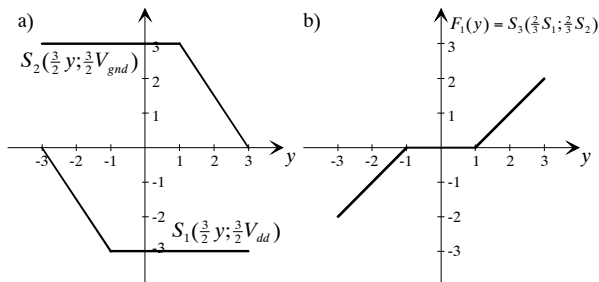
Fig.18 Constructing of the function F_1(y) .
