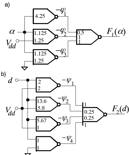
Fig.44 Fuzzifiers of the variables a) angle and b) distance.
