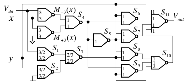
Fig.19 Structural diagram of the controller.
