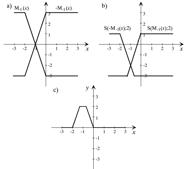
Fig.14 Implementation example of the rule (19).
