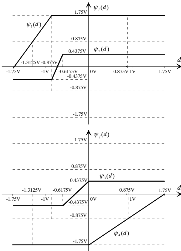
Fig.43 Component functions for the function represented in Fig.42.
