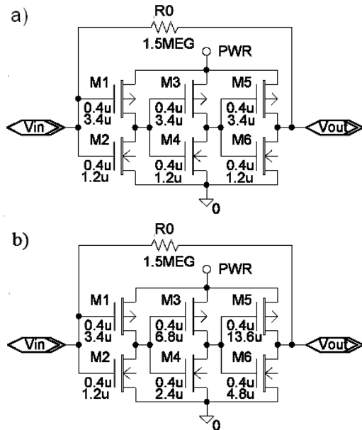
Fig.35 Operational amplifier with feedback: a) ordinary, b) powerful.
