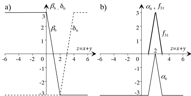
Fig.32 Functional representations of the matrixes M_5 .
