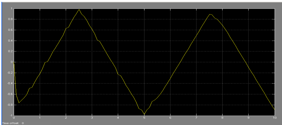
Fig. 15 Gimbal angle output for the integration method with w_1=0.95 and w_2=0.05 and T=0.1 .
