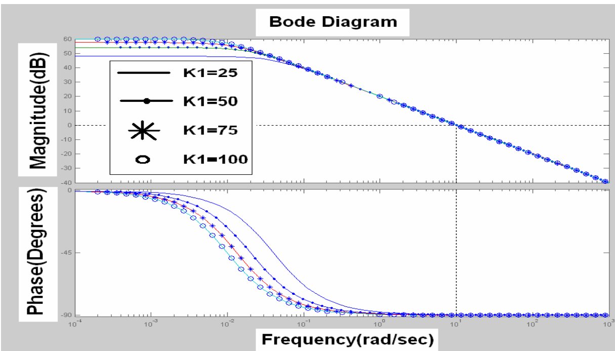
Fig. 5 Bode plots for several K_1 's with T=0.1 and K_0=5 .
