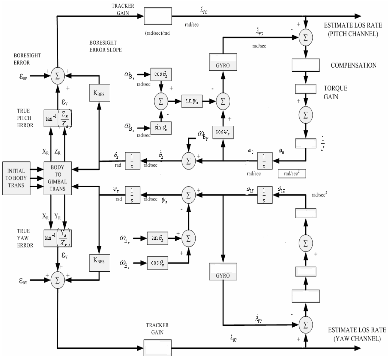
Fig. 1 The detailed block diagrams of antenna tracking and stabilization loops.
