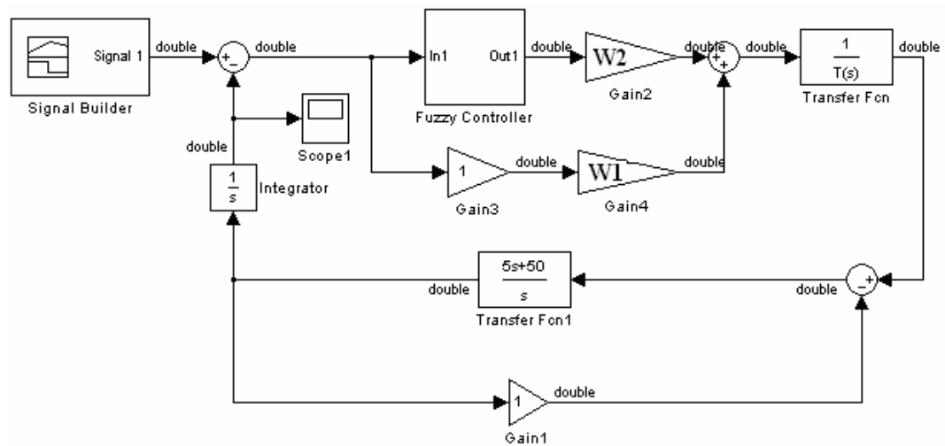
Fig. 14 Integration of traditional and fuzzy controllers by taking the weighting factors respectively as w_1 and w_2 .
