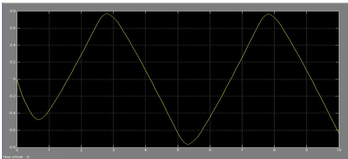
Fig. 16 Gimbal angle output for the integration method with w_1=0.95 and w_2=0.05 and T=1 .
