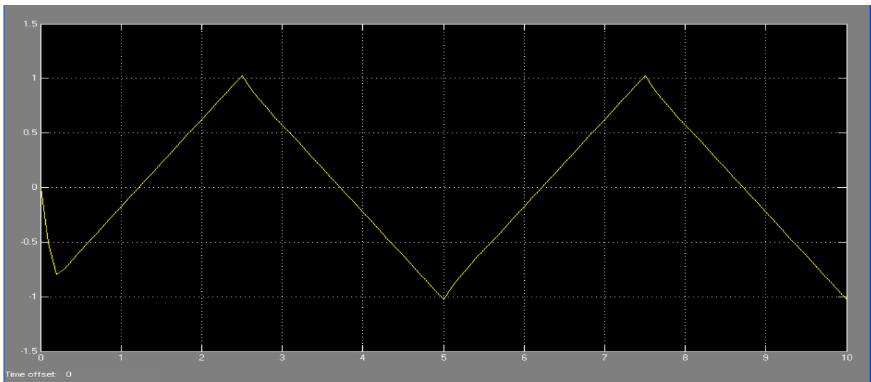
Fig. 18 Gimbal angle output for the integration method with w_1=0.9 and w_2=0.1 and T=0.1 .
