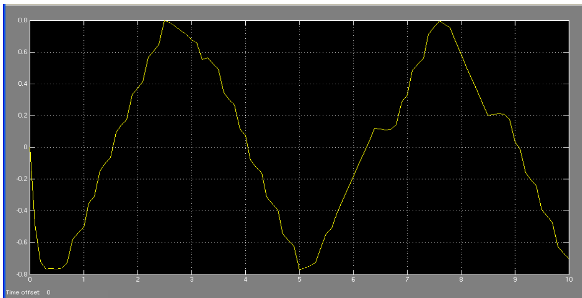
Fig. 12 Gimbal angle output obtained by fuzzy controller with T=1 .
