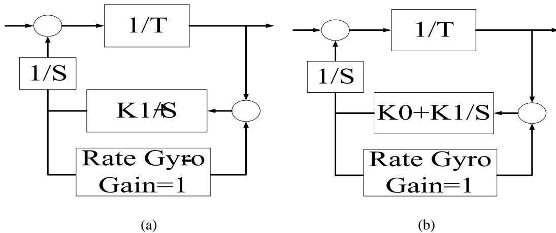
Fig. 2 Simplified block diagrams of antenna pitching or yawing control systems for the stabilization loop applying (a) pure integration, and (b) PI compensators.
