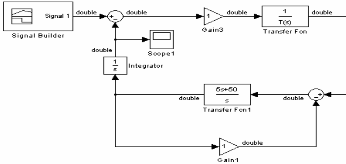
Fig. 6 Antenna performance analyses with traditional design.
