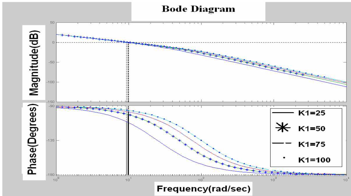
Fig. 3 Bode plots for K_1 are as 25, 50, 75 and 100, respectively.
