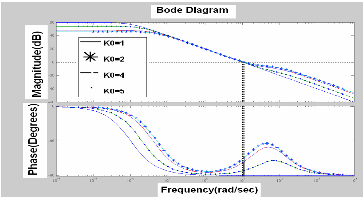
Fig. 4 Bode plots for several K_0 's with T=0.1 and K_1=100 .
