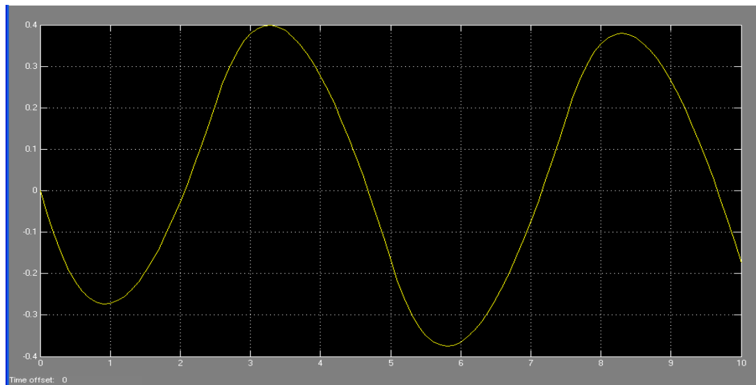
Fig. 10 Gimbal angle output obtained by traditional design with T=1.5 .
