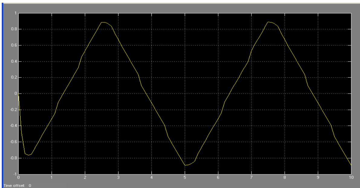
Fig. 13 Gimbal angle output obtained by fuzzy controller with T=1.5 .
