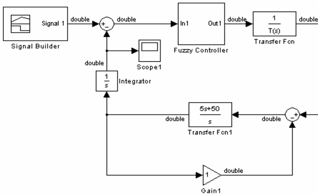
Fig. 11 A fuzzy controller is applied in the tracking loop design.
