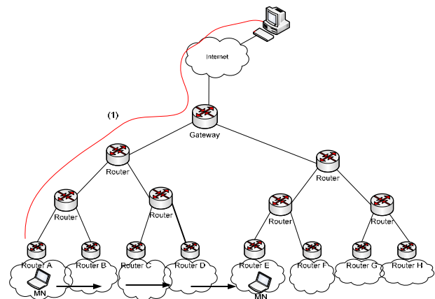
Figure 8: Signaling Path retransmission by PF
