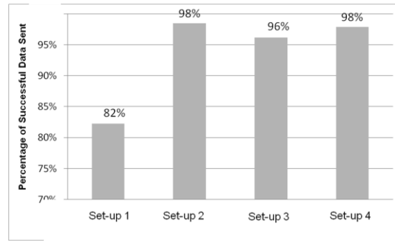
Figure 11: Co-channel interference while transmitting alternately
