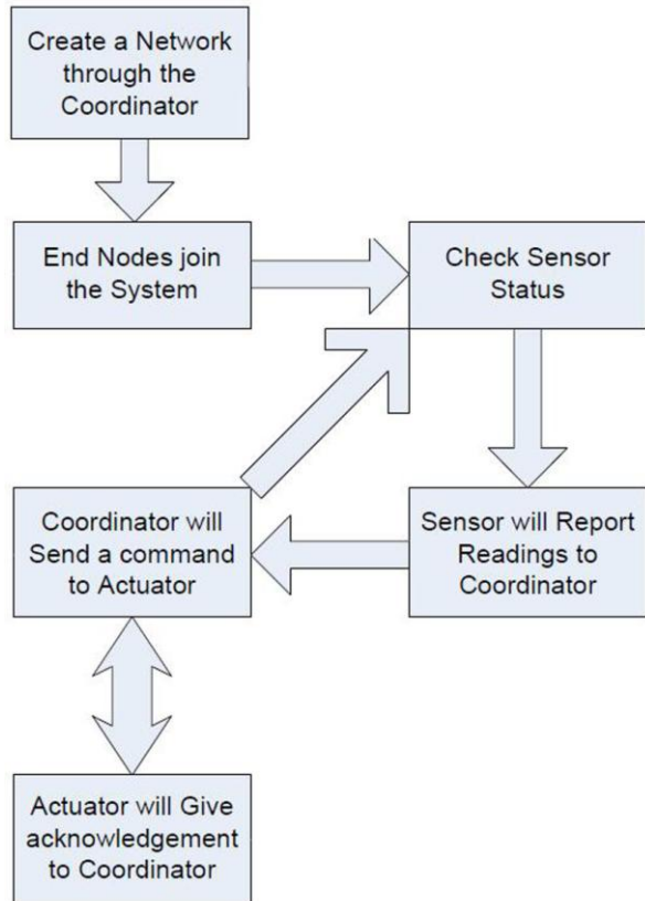
Figure 8: Zigbee-based WSAAN System
