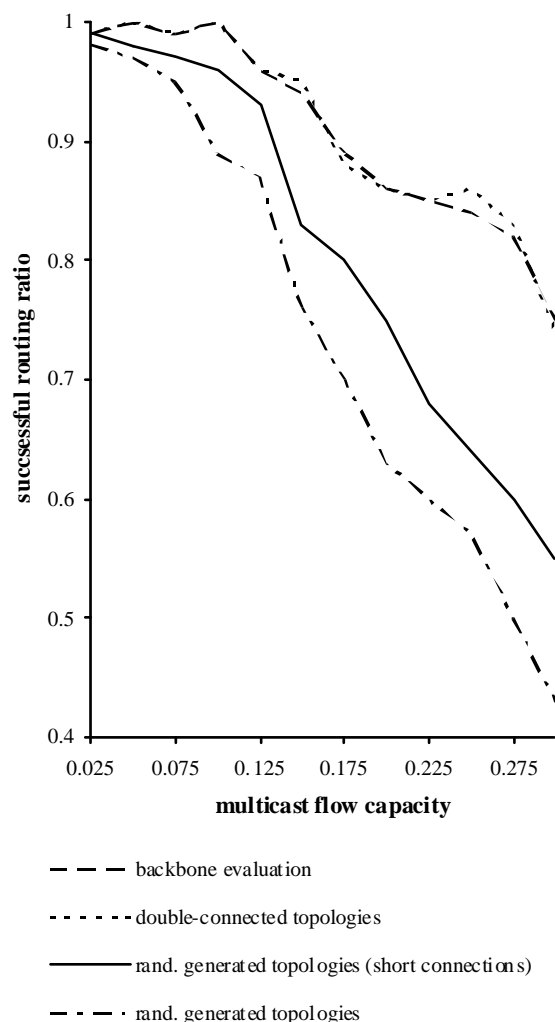
Fig. 4. Successful routing ratio for different types of topologies, using the optimal routing algorithm, 200 paths / point
