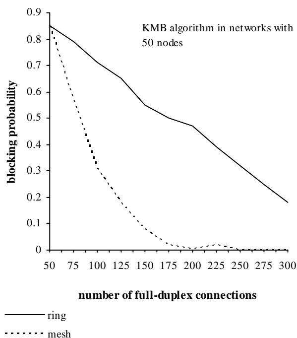
Fig. 14. Networks with 50 nodes, comparison between ring and mesh topologies
