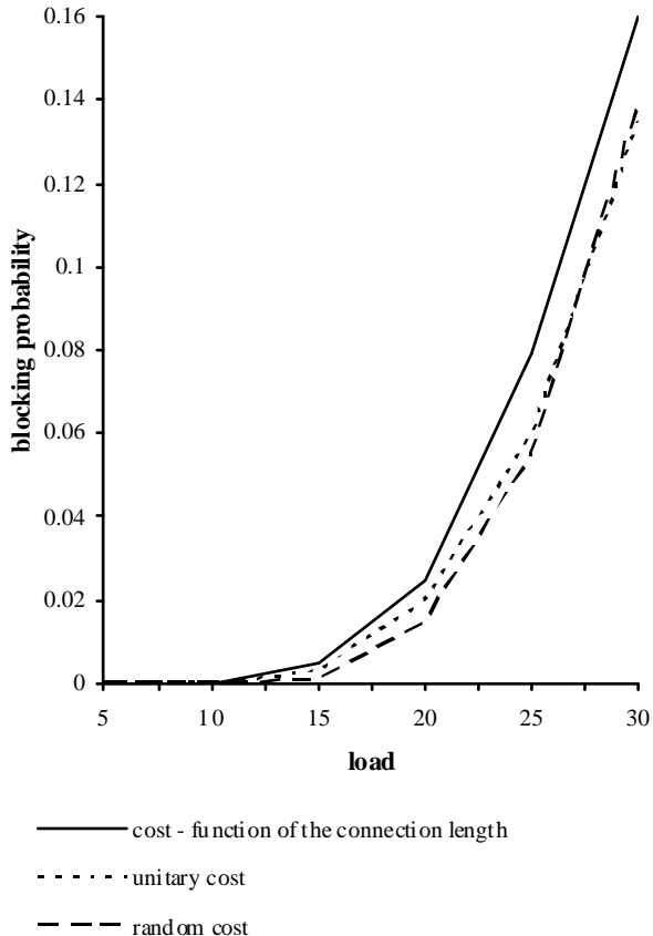
Fig. 15. Non – unitary costs , 25000 routes/point
