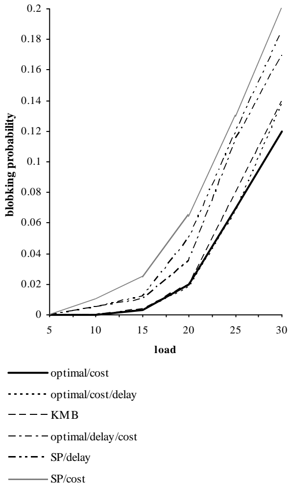
Fig. 8. Blocking probability, single multicast, 5000 paths / point
