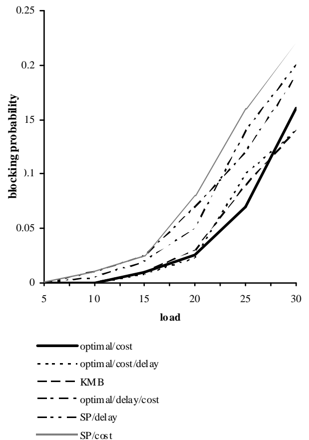
Fig. 7. Blocking probabilities for double connection topologies, with 12 nodes and 15 connections, single multicast sessions, 5000 paths / point
