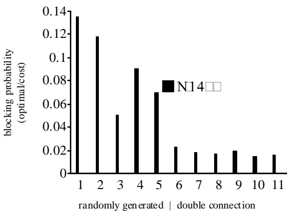
Fig. 6. Blocking probability in randomly generated topologies and in double-connection topologies, 5000 paths / point
