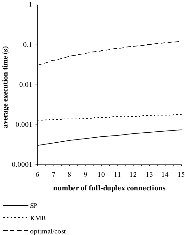
Fig. 16. Execution time for networks with 6 nodes. 15000 routes/point
