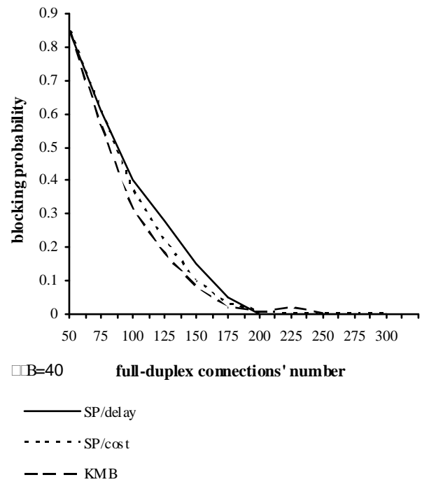
Fig. 13. Networks with 50 nodes, session arrival rate is constant; number of destinations is between 1 and 10 (15 000 paths / point)
