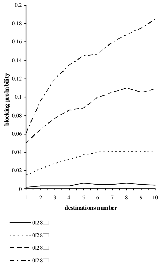
Fig. 9. Blocking probability as a number of destinations for multicasts, optimal/cost algorithm, 10 000 paths / point
