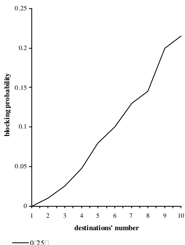
Fig. 10. Blocking probability as a function of the number of destinations in a low load case, with a latency constraint
