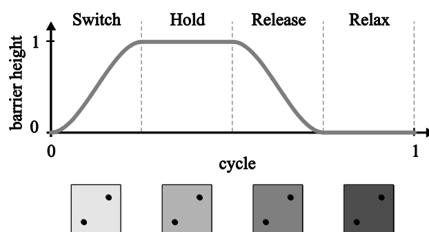
Fig. 2. Graph shows the normalized values of the inter dot barrier height in particular phase of the cyclic clock signal. The value 1 corresponds to the highest barrier. The background shade of the tQCA cell denotes corresponding clock phase assigned to this cell at the beginning of circuit operation. Afterwards the phase shifts through complete cycle.
