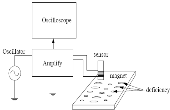
Figure 3 A Nondestructive Test of Metal Imperfection by Using Eddy Current Method
