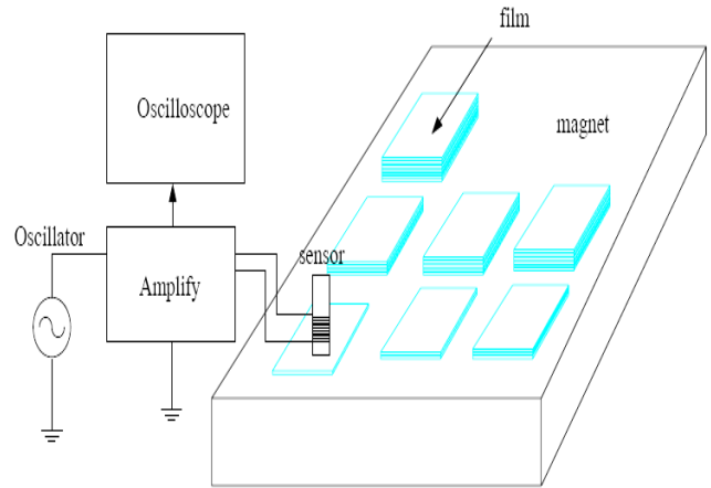
Figure 5. A Nondestructive Test to Find the Thickness of Films on Iron by Using Eddy Current Method
