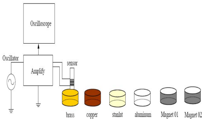
Figure 4. A Nondestructive Test of Metal Categorization by Using Eddy Current Method
