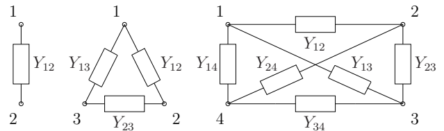
Figure 4: Representation of some n -terminal networks.
