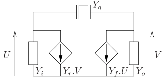
Figure 9: Reduced form of the oscillator.
