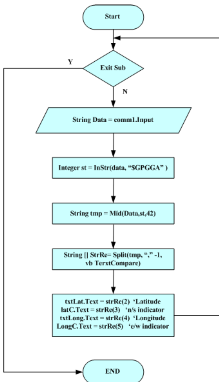
Fig. 11. Algorithm of word cutting from GPS data from GPS receiver engine board.
