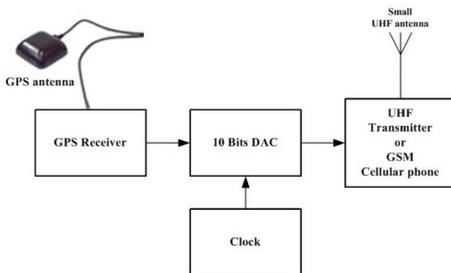
Fig. 7. Block diagram of GPS transmitter System
