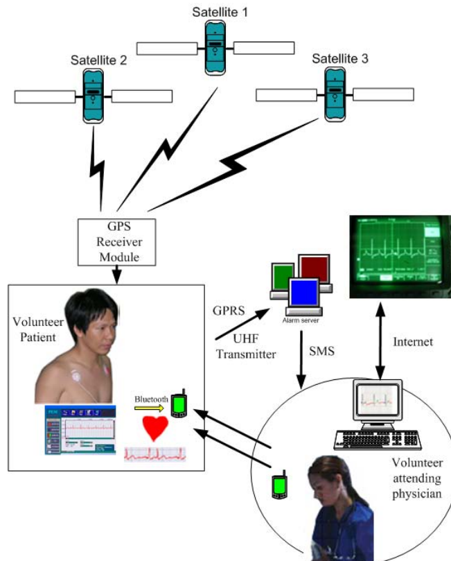
Fig. 3. The structure of overall system.
