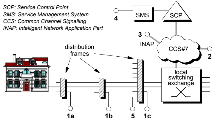
Fig. 1: Scheme of telephone network with possible interconnection points for unbundled services.
