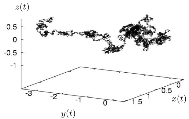
(b) stochastic ODE
