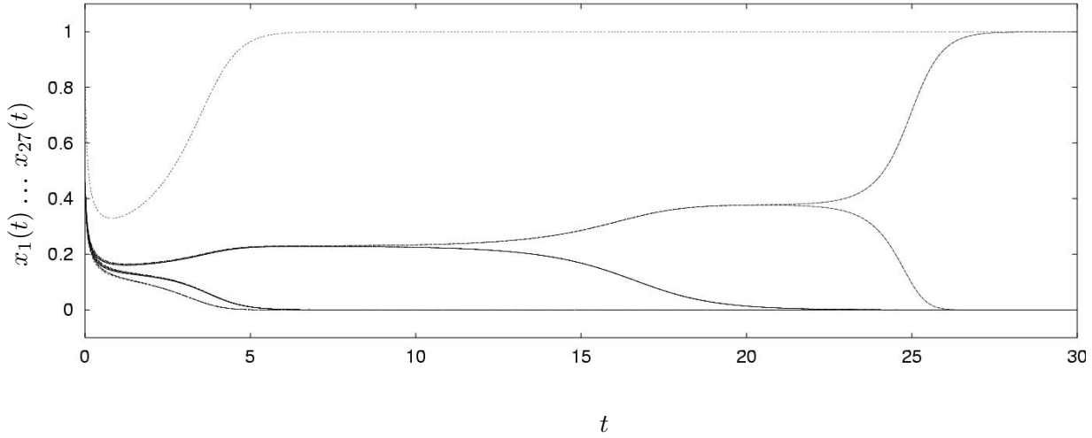
Figure 4: Dynamics of a CODEL, supported by AnT.
