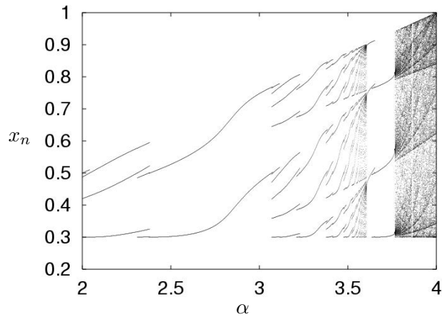
(a) bifurcation diagram
