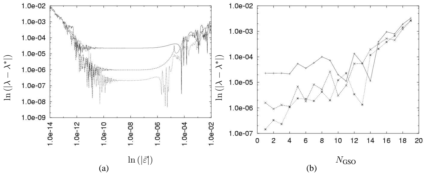
Figure 8: Accuracy of the numerical calculation of the Lyapunov exponents for the logistic map x_{n+1} = \alpha x_n(1 - x_n) for \alpha = 4.0 . The number of iterations is 25 000 steps (solid line), 250 000 steps (dashed line) and 2 500 000 steps (dotted line). The transient part is 1000 steps in all three cases. The initial value is x_0 = 0.1 .
