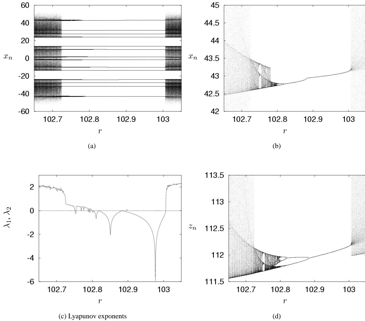
Figure 7: Investigation of the Lorenz–63 system.
