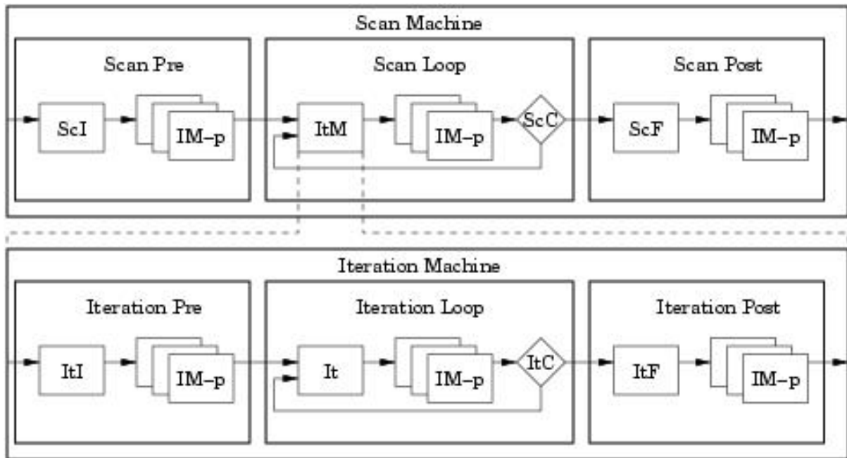
Figure 11: Architecture of the AnT simulator.
