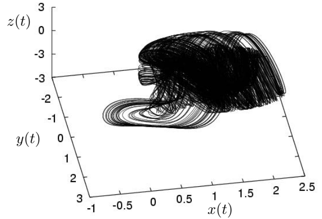
(b) ordinary differential equation
