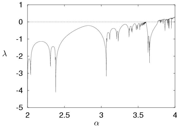
(c) Lyapunov exponent \lambda
