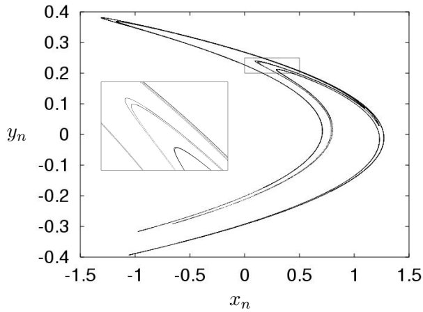
(a) discrete map
