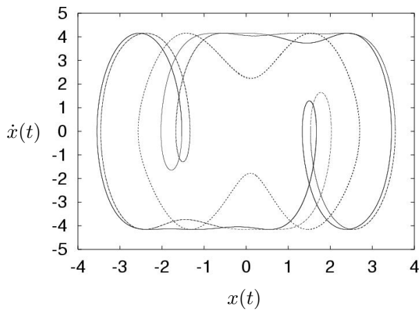
(a) delay differential equation
