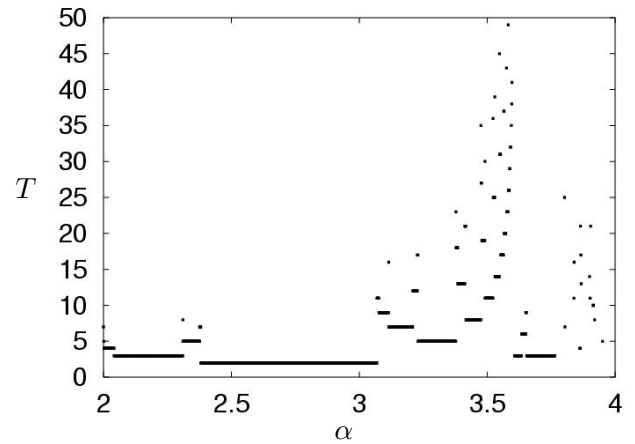
(b) period diagram
