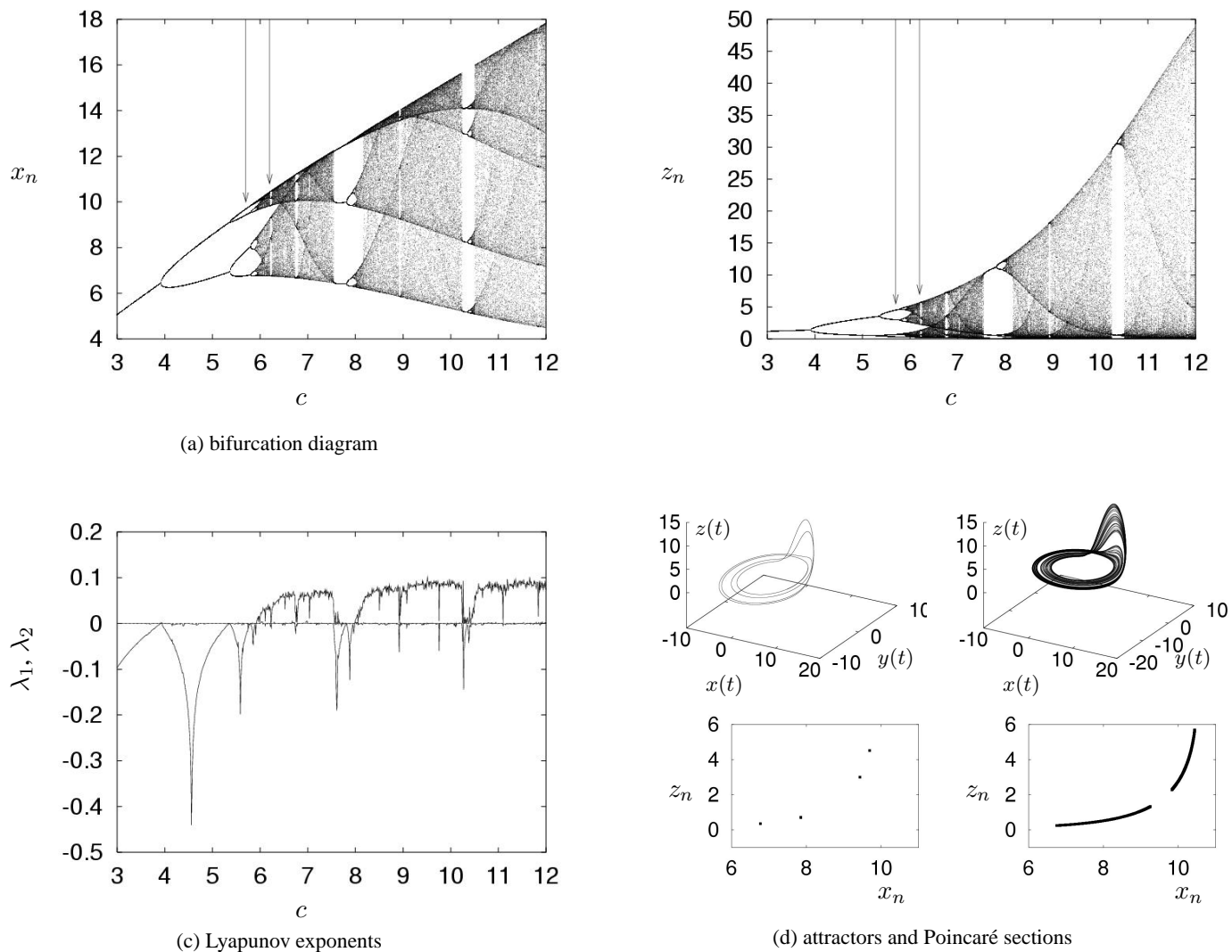
Figure 6: Investigation of the Rössler system.
