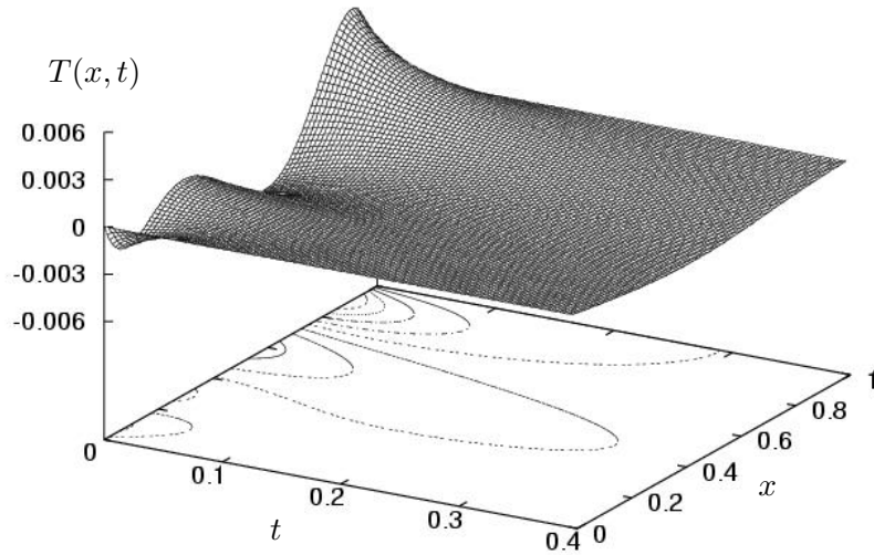
Figure 5: Dynamics of a one dimensional PDE, supported by AnT.
