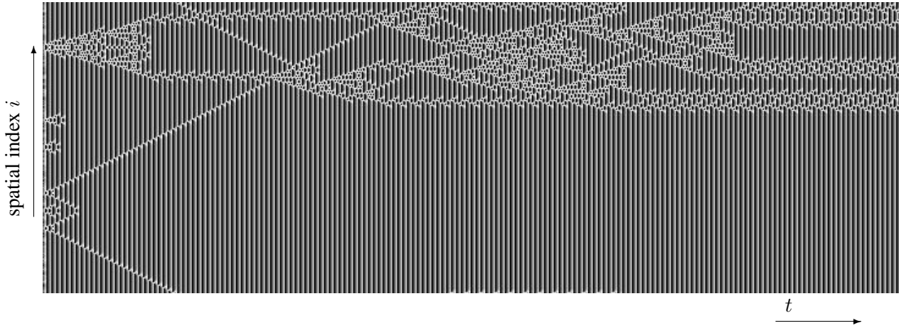
Figure 3: Dynamics of a CML, supported by AnT.
