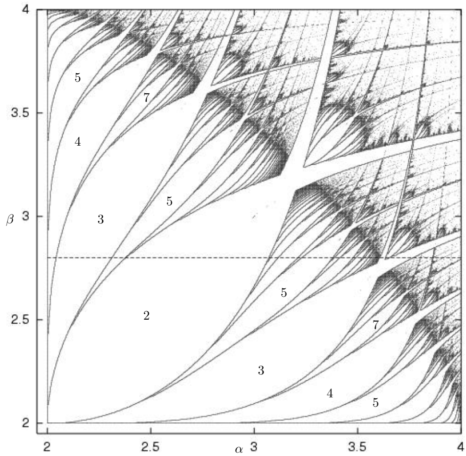
Figure 10: Bifurcation structures of the system (1) in the 2-dimensional parameter space [\alpha \times \beta] .
