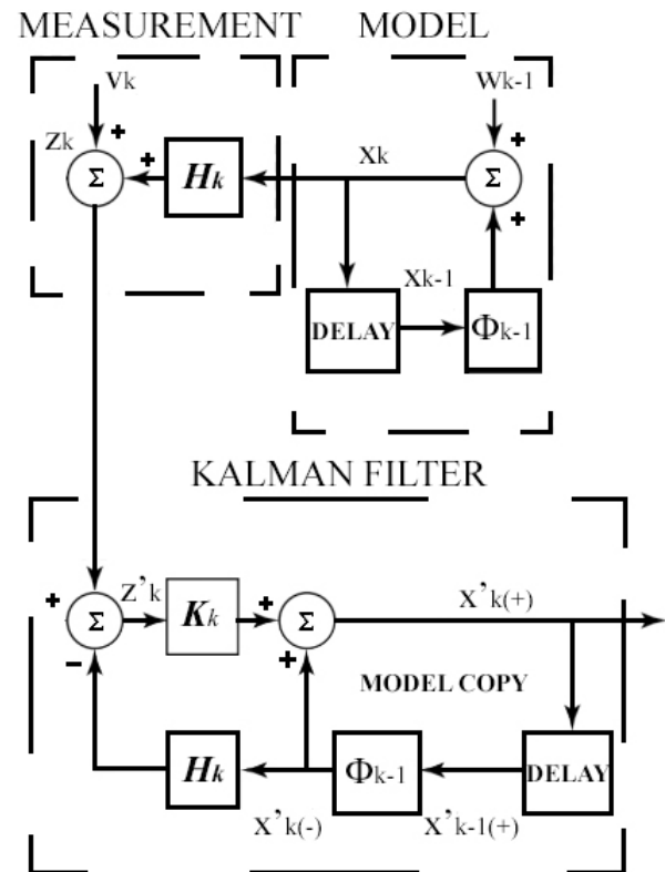
Fig.2 Kalman Filter – Block Diagram
