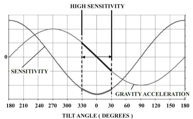
Fig.4 Sensitivity – Tilt relationship
