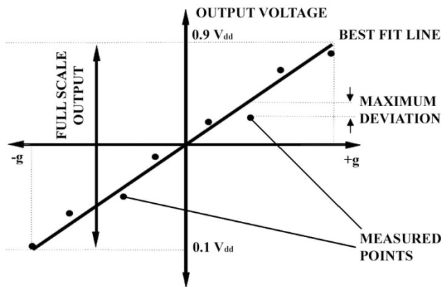
Fig.5 Non-linearity
