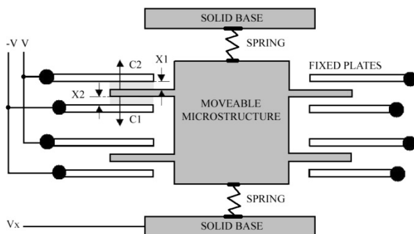
Fig.1 Simplified scheme of MEMS accelerometer
