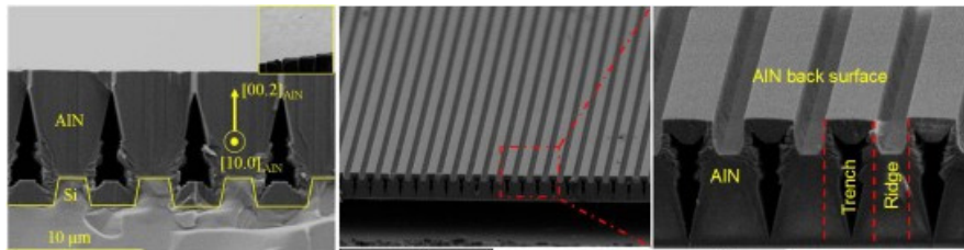
Figure 3. Scanning electron micrographs of the thick AlN growth (left) a side-view of the regrowth with yellow lines delineating the boundary between the AlN growth and the silicon substrate; and, (middle & right) an inclined view of the surface after flip-chip bonding and substrate removal.
