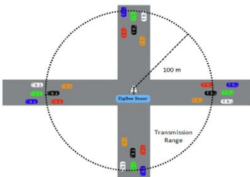
Fig. 2 The design of the network in Qualnet simulator
