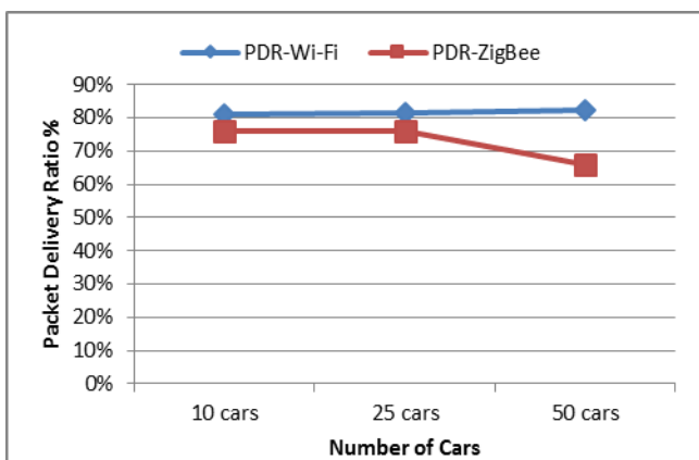
Fig. 6 The packet delivery ratio of ITS using ZigBee and Wi-Fi
