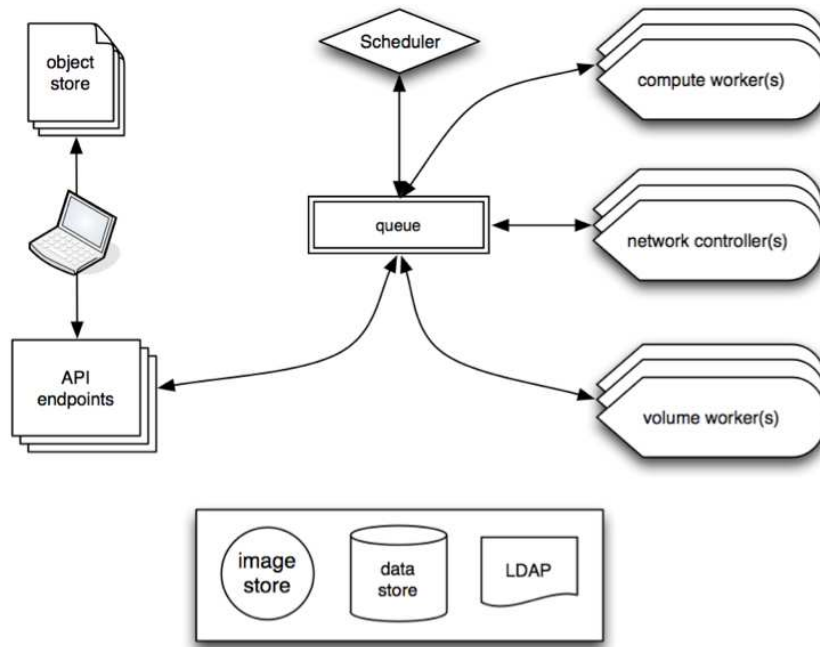
Figure 3: Nova system architecture [10].
