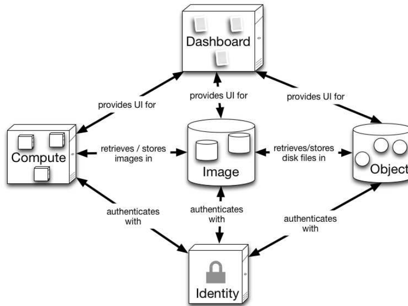
Figure 2: OpenStack Architecture [10].
