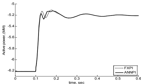
Fig. 10. Active power flow between source and WECS sides connected by two lines, case 3.
