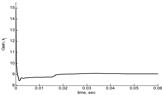
Fig. 5. First updating for k_i in controller 1.
