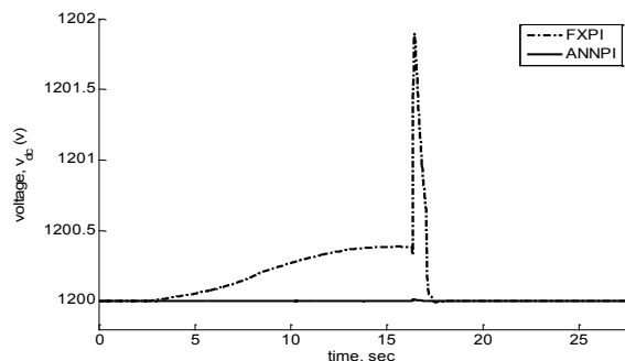
Fig. 6. DC link voltage performance, case 2.
