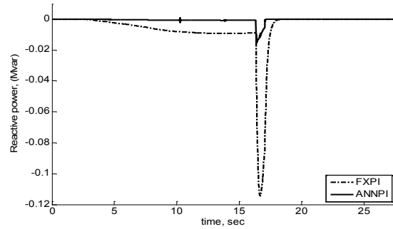
Fig. 7. Reactive power exchange, case 2.
