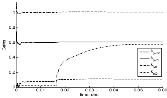
Fig. 4. Gains in controllers for v_{dc} , v_d and Q .
