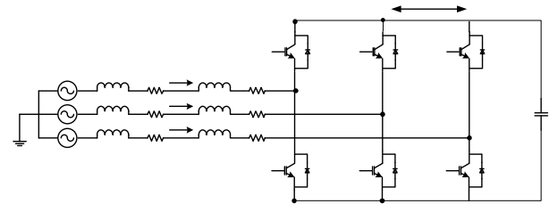
Fig. 2. Voltage source converter model.
