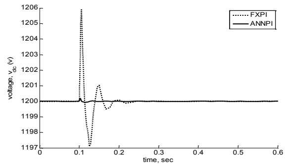
Fig. 8. DC link voltage performance, case 3.
