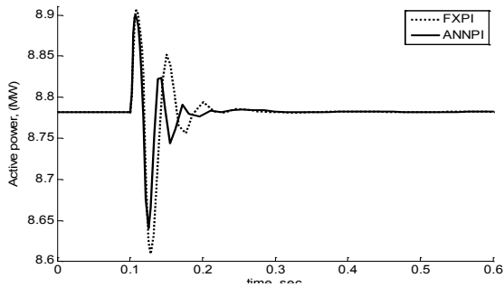
Fig. 9. Active power in WECS terminals, case 3.
