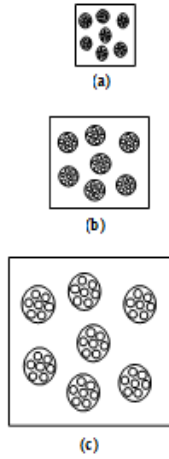
Fig. 15 Effects of internal versus external potential energy as the system volume is increased.
