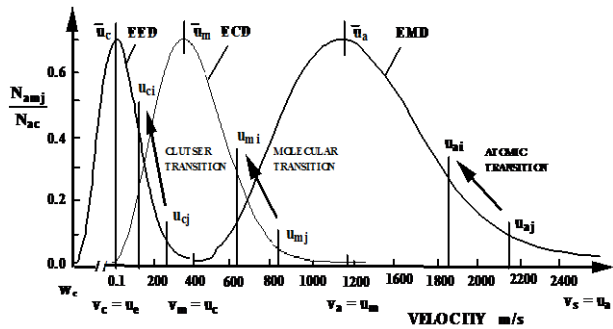
Fig. 16 Maxwell-Boltzmann speed distribution viewed as stationary spectra of cluster sizes for EED, ECD, and EMD scales at 300 K [33].
