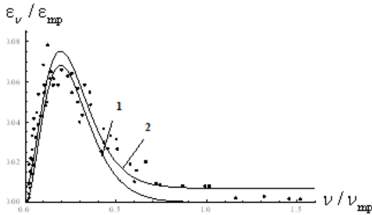
Fig. 8 One-dimensional dissipation spectrum [100] compared with (1) Planck energy distribution (2) Planck energy distribution with constant displacement. 2
