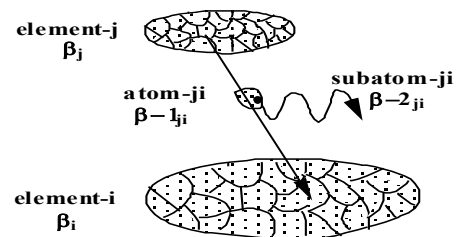
Fig. 20 Transition of “atom” a_{ij} from element- j to element- i leading to emission of sub-atomic particle s_{ij} .
