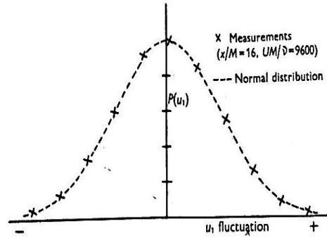
Fig. 5 Measured velocity distribution in isotropic turbulent flow [58].
