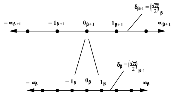
Fig. 18 Hierarchy of normalized coordinates associated with embedded statistical fields [122].
