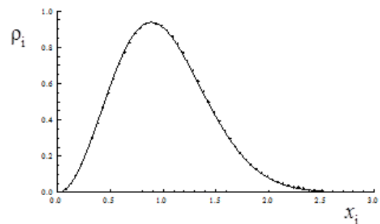
Fig. 17 Probability density of normalized spacing between zeros of Riemann zeta function [125] \gamma_n, 10^{12} \leq n \leq 10^{12} + 10^5 , normalized spacing between
