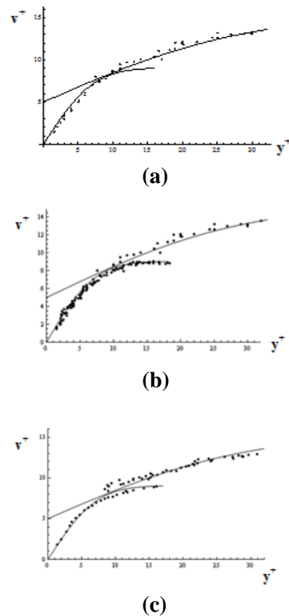
Fig. 3 Comparison between the predicted velocity profiles (a) LED-LCD, (b) LCD-LMD, (c) LCD-LAD with experimental data in the literature over 10^8 range of spatial scales [35].
