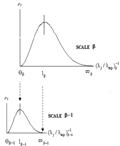
Fig. 14 Maxwell-Boltzmann speed distribution as a function of oscillator wavelengths (\lambda_j/\lambda_{mp})^{-1} .
