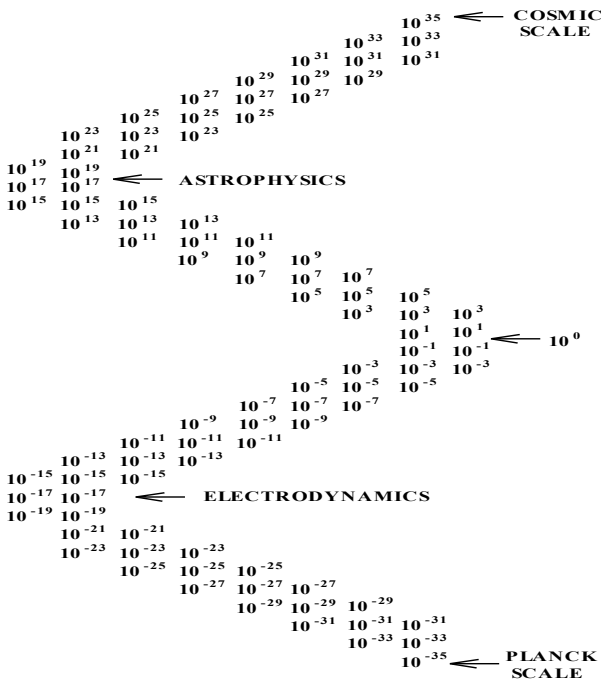
Fig. 4 Hierarchy of statistical fields with (\ell_\beta, \lambda_\beta, L_\beta) from cosmic to Planck scales [34].
