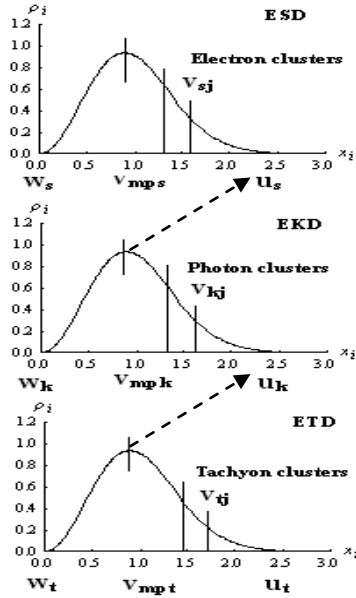
Fig. 13 Maxwell-Boltzmann speed distribution for ESD, EKD, and ETD fields.
