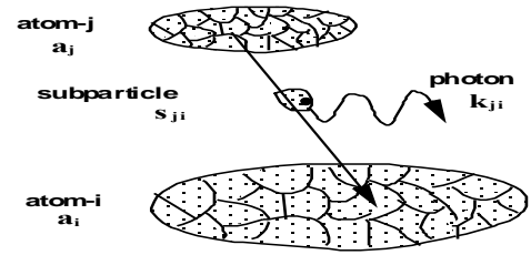
Fig. 19 Transition of electron e_{ij} from atom- j to atom- i leading to emission of photon k_{ij} [51].
