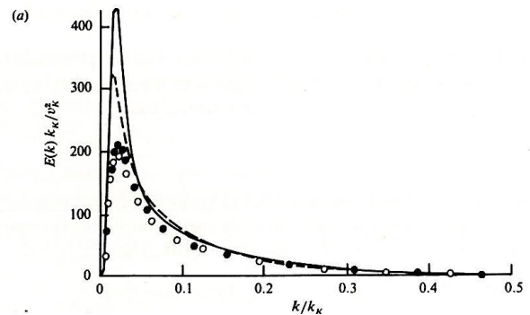
Fig. 7 Normalized three-dimensional energy spectra for isotropic turbulence [98].
