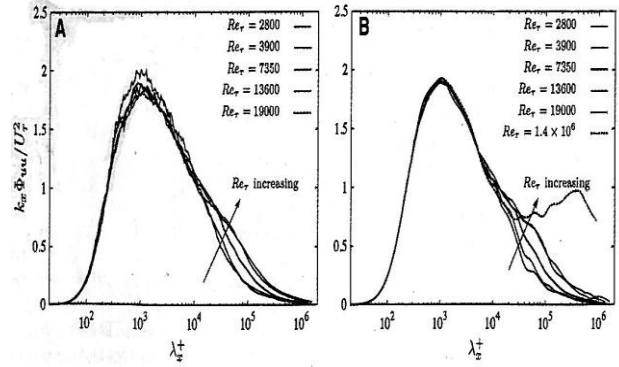
Fig. 10 Reynolds number evolution of the pre-multiplied energy spectra of stream wise velocity at the inner-peak location ( z^+ = 15 ) for the true measurements (A) and the prediction based on the filtered u signal measured in the log region (B) [102].
