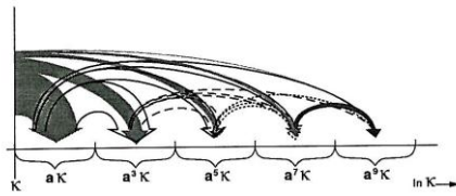
Fig.11 A realistic view of spectral energy flux [105].
