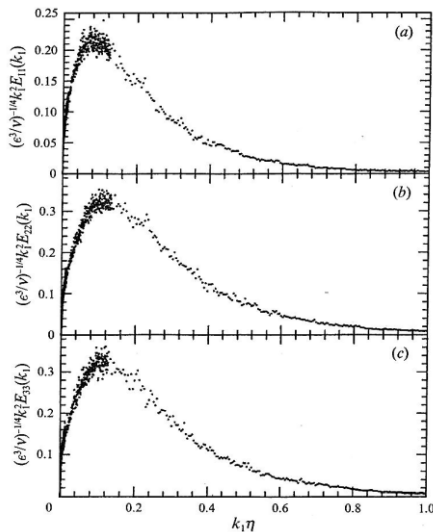
Fig. 9 One-dimensional dissipation spectra (a) u_1 -spectrum (b) u_2 -spectrum (c) u_3 -spectrum [101].
