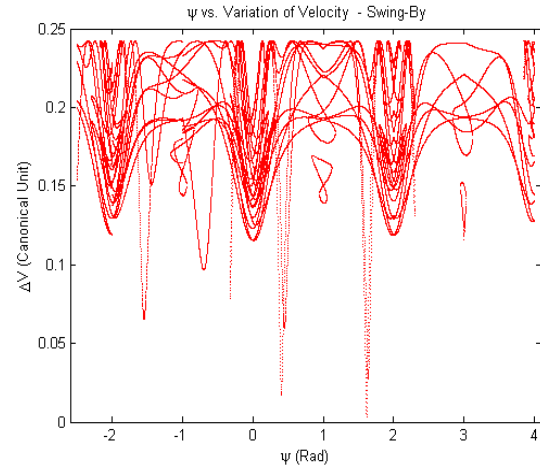
Figure 4 - \psi vs. Variation of velocity ( \Delta V ), for e = 0.4 , \psi_0 = -2.5 rad \psi_f = 4 rad.
