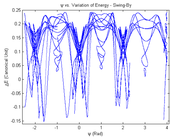
Figure 6 - \psi vs. Variation of Energy ( \Delta E ), for e = 0.4 , \psi_0 = -2.5 rad \psi_f = 4 rad.
