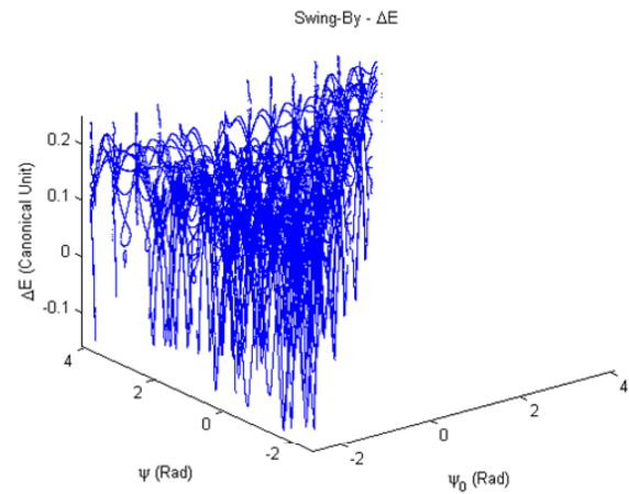
Figure 5 - Variation of Energy ( \Delta E ) after the Swing-By with e = 0.4 , \psi_0 = -2.5 rad \psi_f = 4 rad.
