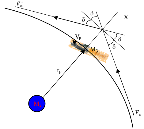
Figure 1 – Swing-By Maneuver.
