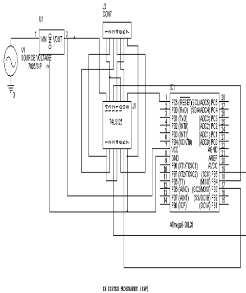
Fig.2 In System Programmer
