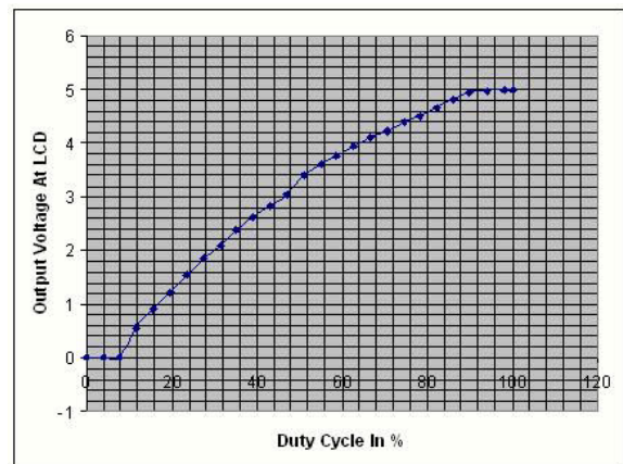
Fig3: Duty cycle vs. Output voltage
