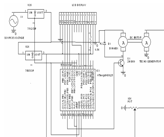
Fig. 1 Motor Controller Sections
