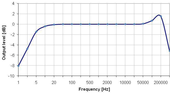
Fig. 4, Rectifier frequency response
