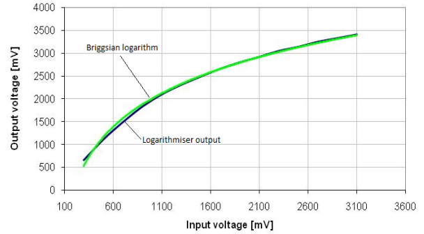
Fig. 5, Logarithmiser performance
