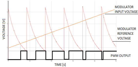
Fig. 1, PWM modulator waveforms
