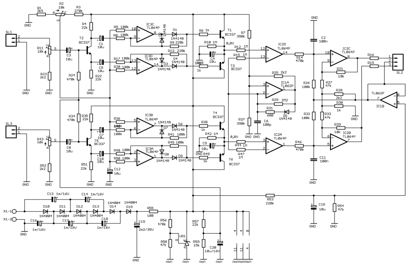
Fig. 6, Complex two-channel VU meters driver
