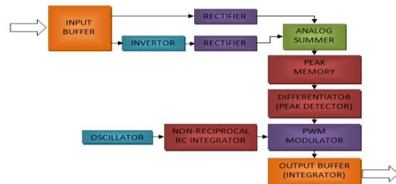
Fig. 2, Basic blocks of the sample rectifier and logarithmic driver
