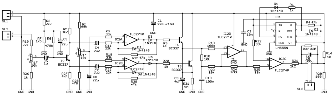
Fig. 3, Sample circuit schematics
