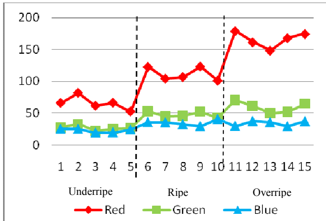
Fig. 14: RGB values for underripe, ripe and overripe of training image.
