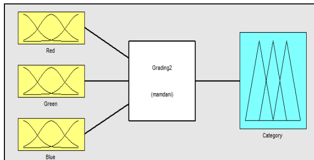
Fig. 8: The Fuzzy Inference System consists of three inputs and one output.
