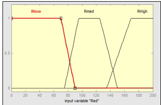
Fig. 9: The Membership Function representation of red input.
