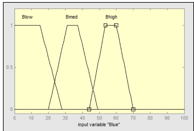
Fig. 11: The Membership Function representation of blue input.
