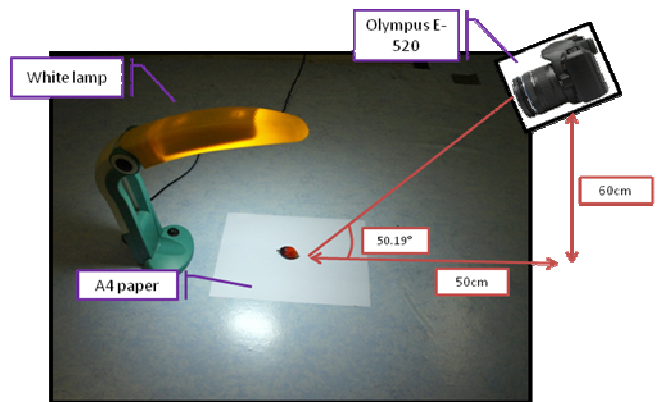
Fig. 2: The image acquisition setup
