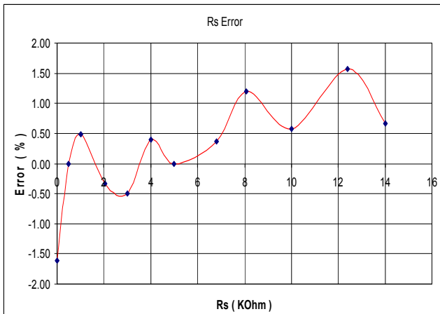
Fig.11 Error percentage of the resistance measurement
