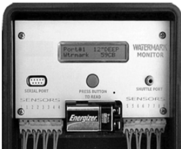
Fig.1 Digital Controller
