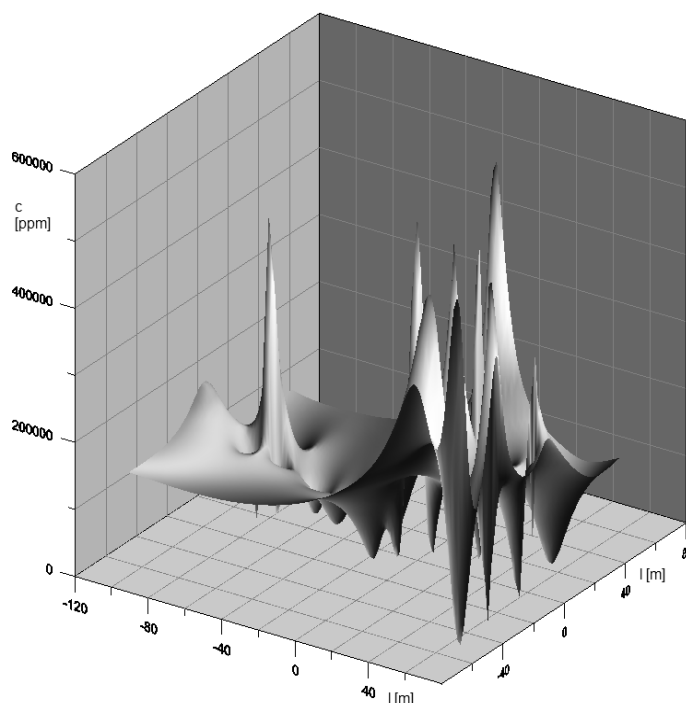
Fig. 2 A 3D-visualization of measured values of the concentration of CO 2 at the municipal waste landfill site.
