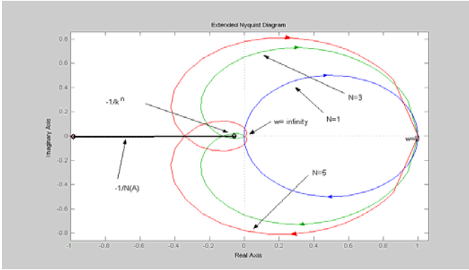
Figure 9: (a) The Extended Nyquist Diagram for Ring Oscillators (N=1,3,5)
