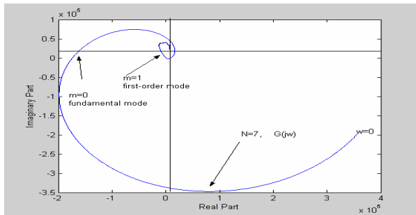
Figure 9: (b) The Extended Nyquist Diagram for Ring Oscillators (N=7)
