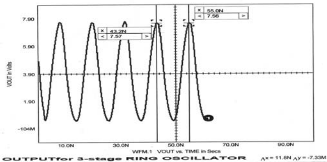
Figure11: Simulation of Period for 3-Stage Ring Oscillator T=11.8 ns
