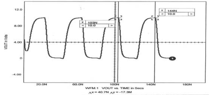
Figure14: Simulation of Period for 9-Stage Ring Oscillator T=40.7 ns
