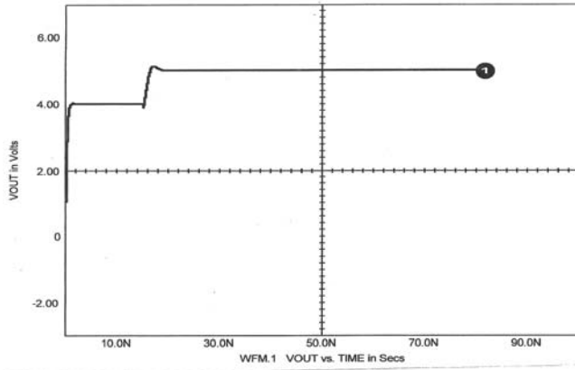
Figure16: Simulation for a 3-stage NMOS Ring Oscillator (Example 2)
