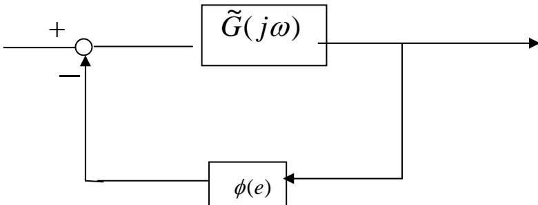
Figure 3: A Conventional Lur'e Problem
