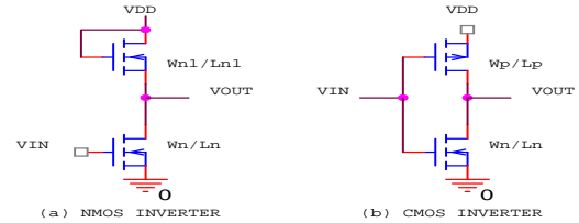
Figure 6: The schematics of NMOS and CMOS inverters
