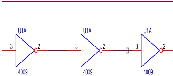
Figure 1: Three-stage Ring Oscillator Circuit Consisting of Identical Inverters
