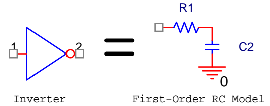
Figure 5: Simplified first-Order RC Model for an Inverter
