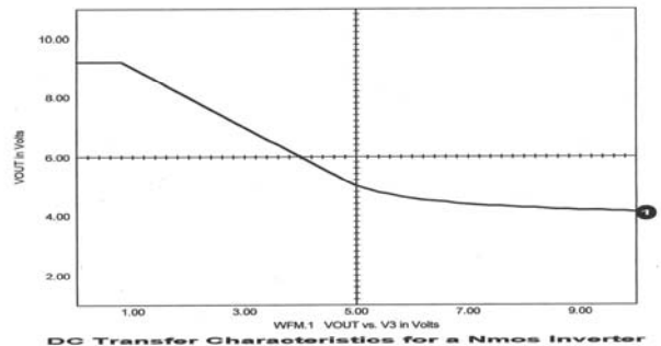
Figure15: DC Input/Output Transfer Characteristic for A NMOS Inverter
