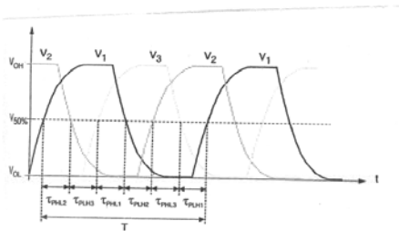
Figure 2: Typical Voltage Waveform of the Three Inverter shown in Fig.1
