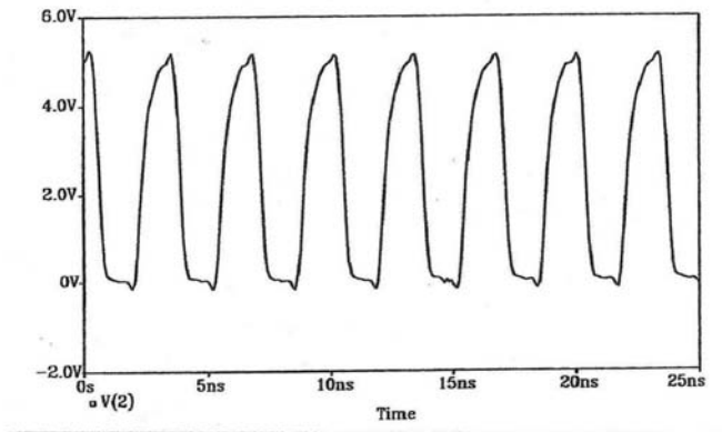
Figure 17: Simulation for a 5-stage Ring Oscillator (CN20 Process)
