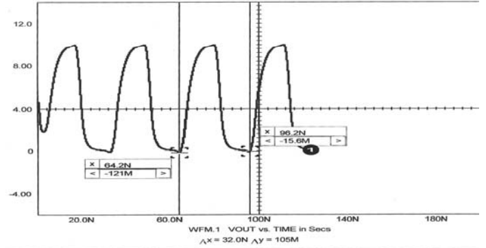
Figure13: Simulation of Period for 7-Stage Ring Oscillator T=32 ns
