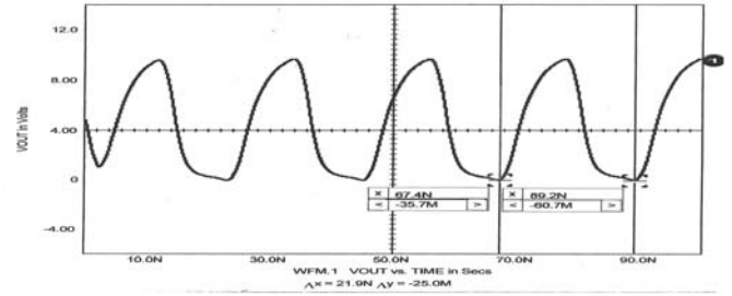
Figure12: Simulation of Period for 5-Stage Ring Oscillator T=21.9 ns
