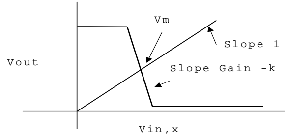
Figure 4: Input-Output (Transfer DC) Characteristics for an Inverter
