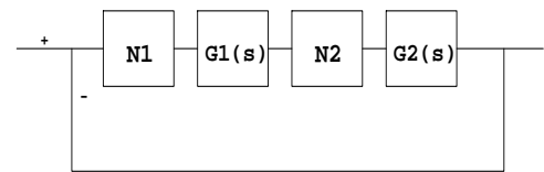
Figure 8: General Multiple Nonlinearity Systems
