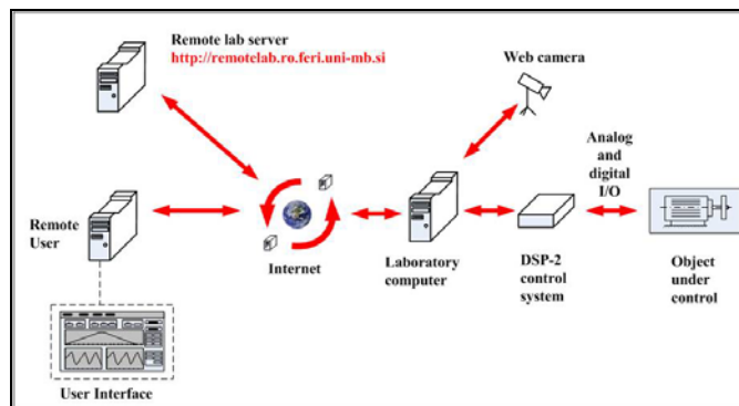
Fig. 1: Architecture of the Remote Laboratory
