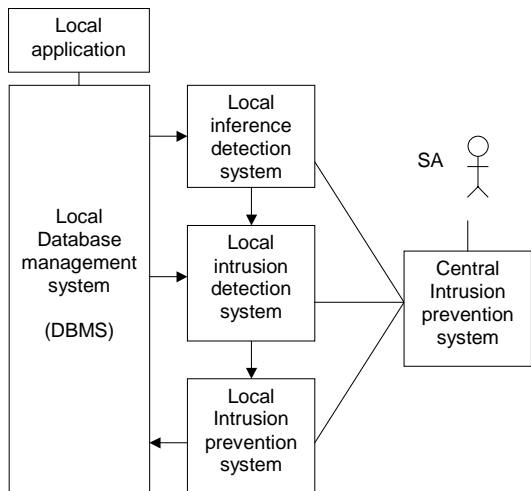
Fig. Intrusion Prevention System connected to a Database System.
