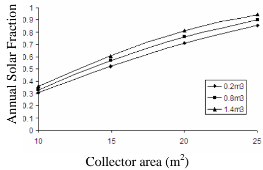
Fig. 7 Annual solar fraction predicted curve as function of solar collector area.
