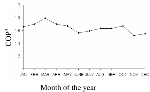
Fig. 8 Monthly coefficient of performance predicted curve for a collector of 10 m 2 area and storage tank size of 0.2 m 3
