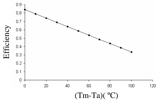
Fig. 3 Characteristics curve of vacuum tube with the temperature difference of mean collector temperature and ambient temperature.
