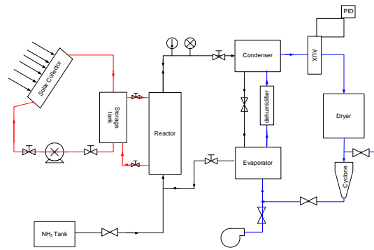
Fig.1 Schematic diagram of solar assisted chemical heat pump dryer
