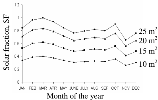
Fig. 6 Monthly solar fraction predicted curve as function of solar collector area
