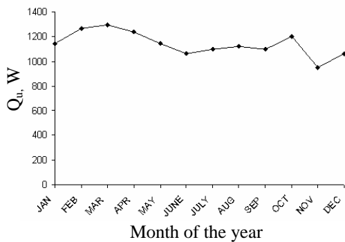
Fig. 5 Monthly useful energy predicted curve
