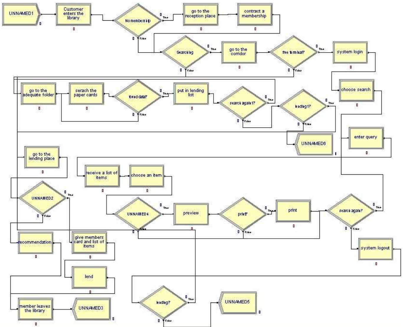
Fig. 4 Library. Example of ARENA simulation model.
