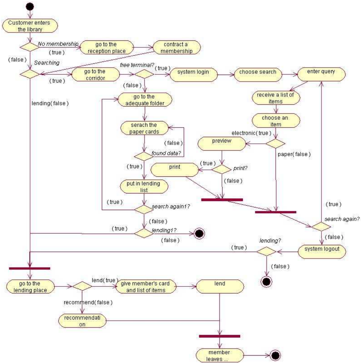
Fig. 3 Library. Example of UML Activity diagram.
