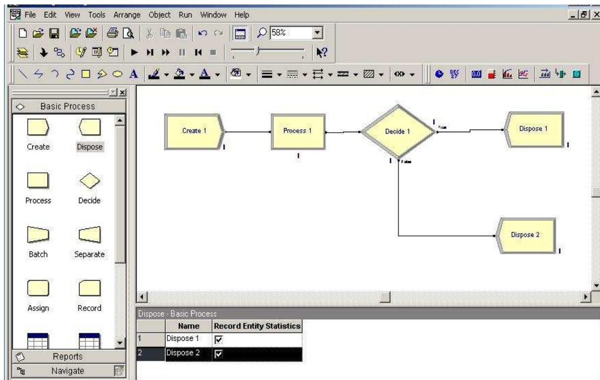
Fig. 2 Model in the Arena simulation environment
