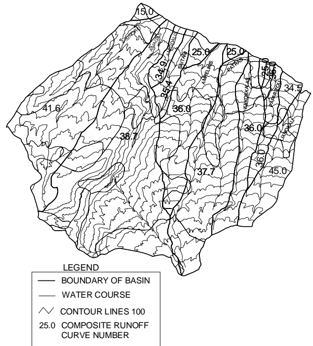
Fig. 4: Map of composite runoff curve numbers CN_c per watershed. Scale 1:80,000
