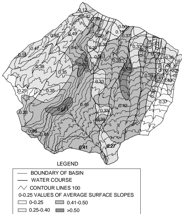
Fig. 3: Map of average surface slopes per category of soil cover. Scale 1:80,000
