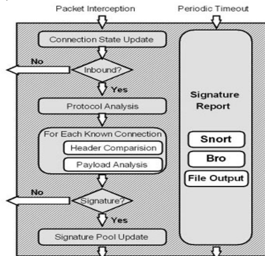
Figure 4: Signature Creation Algorithm [4]
